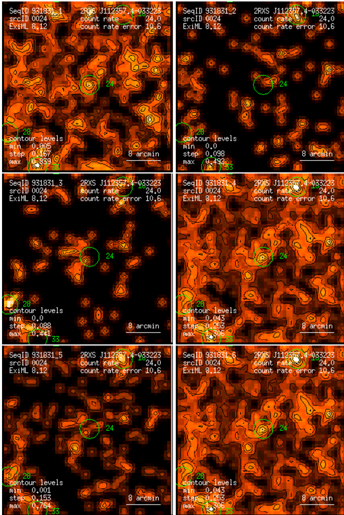
Figure 24: RASS 931831: detection 0024: band rate images, Gaussian filter: (1) PSPC channels 11 – 41, (2) 52 – 90, (3) 91 – 201, (4) 11 – 235, (5) 52 – 201, (6) 11 – 201. Broad band rates in counts/ks. Band rate contour levels in counts/ks/arcmin 2 .
