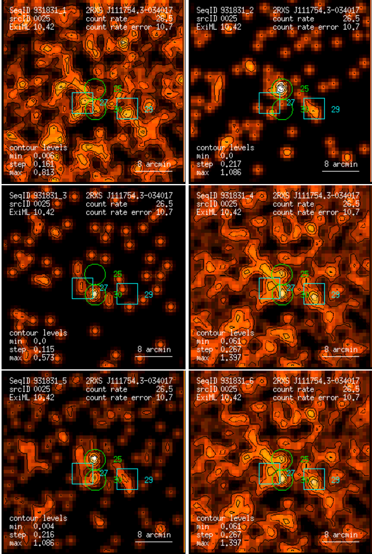
Figure 25: RASS 931831: detection 0025: band rate images, Gaussian filter: (1) PSPC channels 11 – 41, (2) 52 – 90, (3) 91 – 201, (4) 11 – 235, (5) 52 – 201, (6) 11 – 201. Broad band rates in counts/ks. Band rate contour levels in counts/ks/arcmin 2 .
