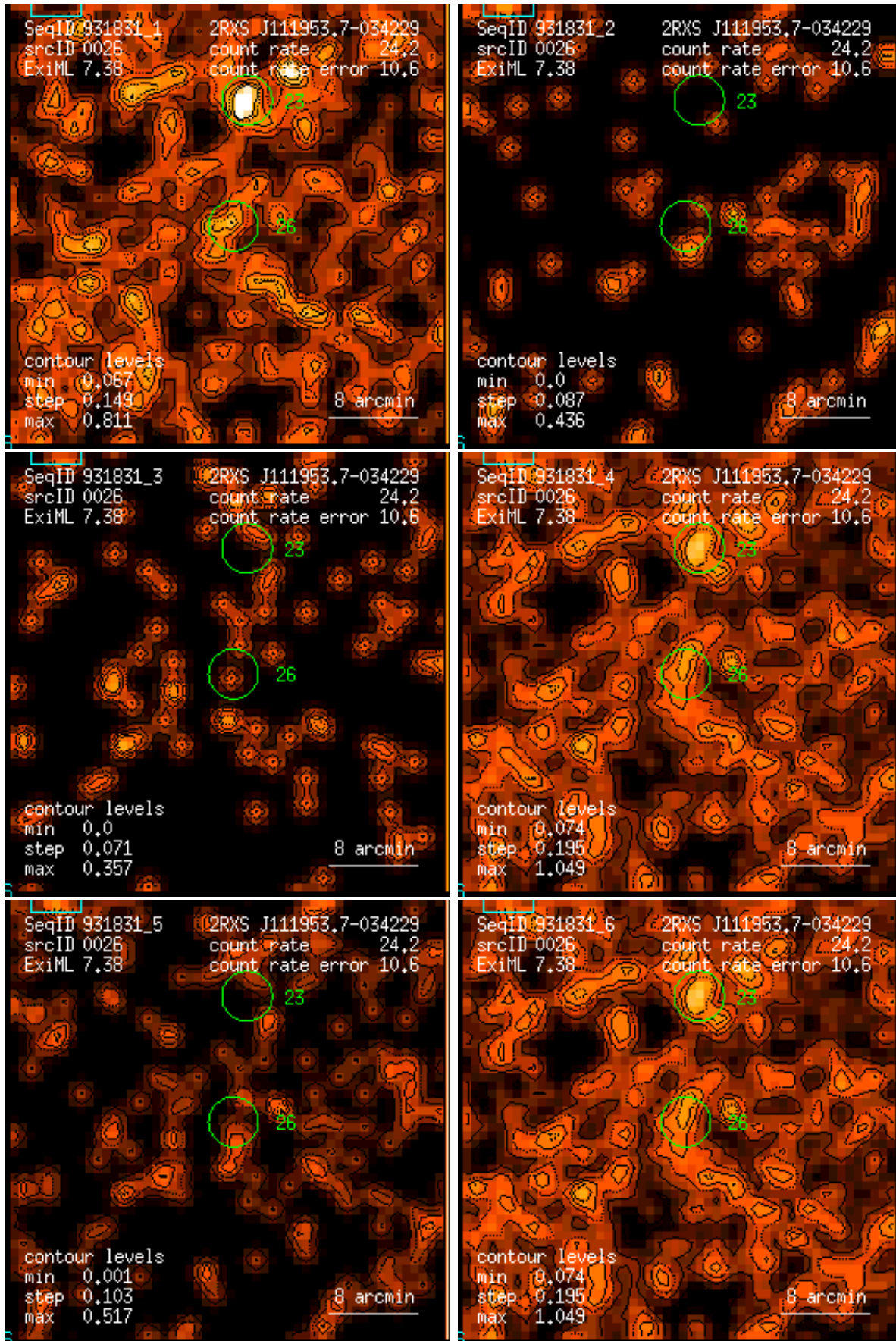
Figure 26: RASS 931831: detection 0026: band rate images, Gaussian filter: (1) PSPC channels 11 – 41, (2) 52 – 90, (3) 91 – 201, (4) 11 – 235, (5) 52 – 201, (6) 11 – 201. Broad band rates in counts/ks. Band rate contour levels in counts/ks/arcmin 2 .
