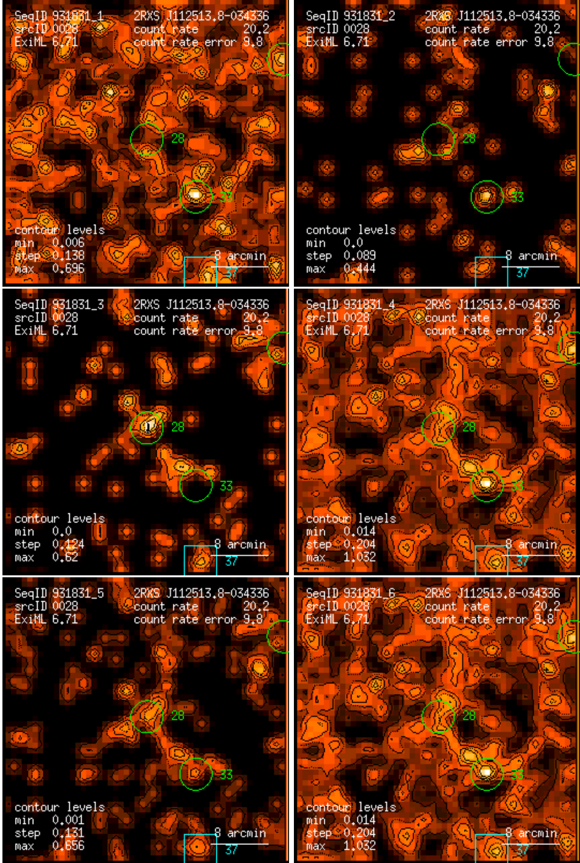
Figure 28: RASS 931831: detection 0028: band rate images, Gaussian filter: (1) PSPC channels 11 – 41, (2) 52 – 90, (3) 91 – 201, (4) 11 – 235, (5) 52 – 201, (6) 11 – 201. Broad band rates in counts/ks. Band rate contour levels in counts/ks/arcmin 2 .
