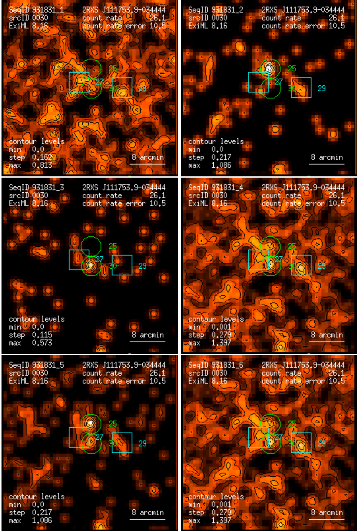
Figure 30: RASS 931831: detection 0030: band rate images, Gaussian filter: (1) PSPC channels 11 – 41, (2) 52 – 90, (3) 91 – 201, (4) 11 – 235, (5) 52 – 201, (6) 11 – 201. Broad band rates in counts/ks. Band rate contour levels in counts/ks/arcmin 2 .
