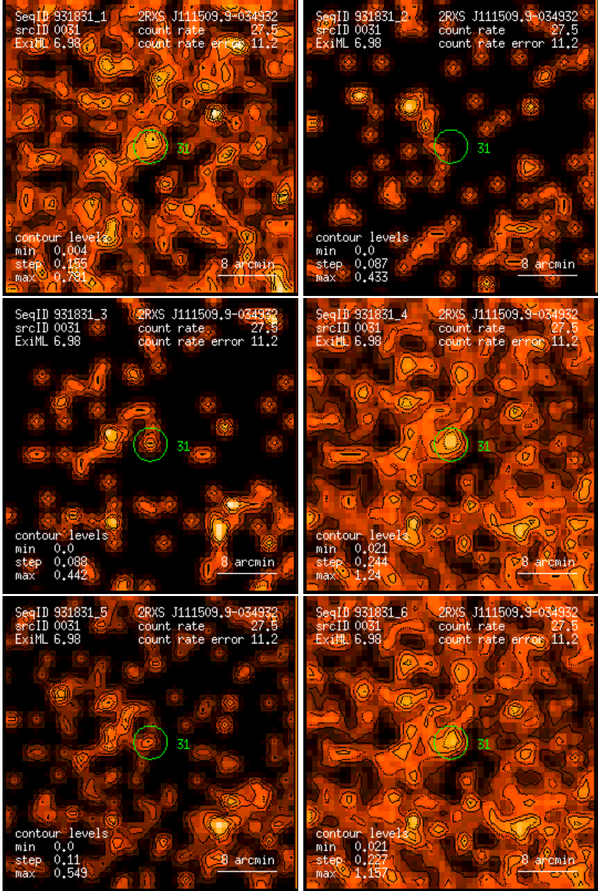
Figure 31: RASS 931831: detection 0031: band rate images, Gaussian filter: (1) PSPC channels 11 – 41, (2) 52 – 90, (3) 91 – 201, (4) 11 – 235, (5) 52 – 201, (6) 11 – 201. Broad band rates in counts/ks. Band rate contour levels in counts/ks/arcmin 2 .
