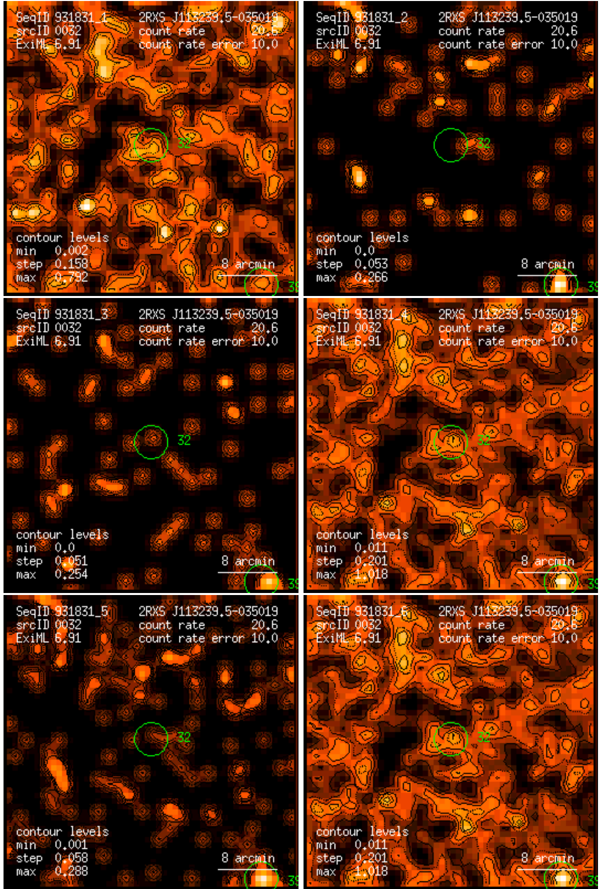
Figure 32: RASS 931831: detection 0032: band rate images, Gaussian filter: (1) PSPC channels 11 – 41, (2) 52 – 90, (3) 91 – 201, (4) 11 – 235, (5) 52 – 201, (6) 11 – 201. Broad band rates in counts/ks. Band rate contour levels in counts/ks/arcmin 2 .
