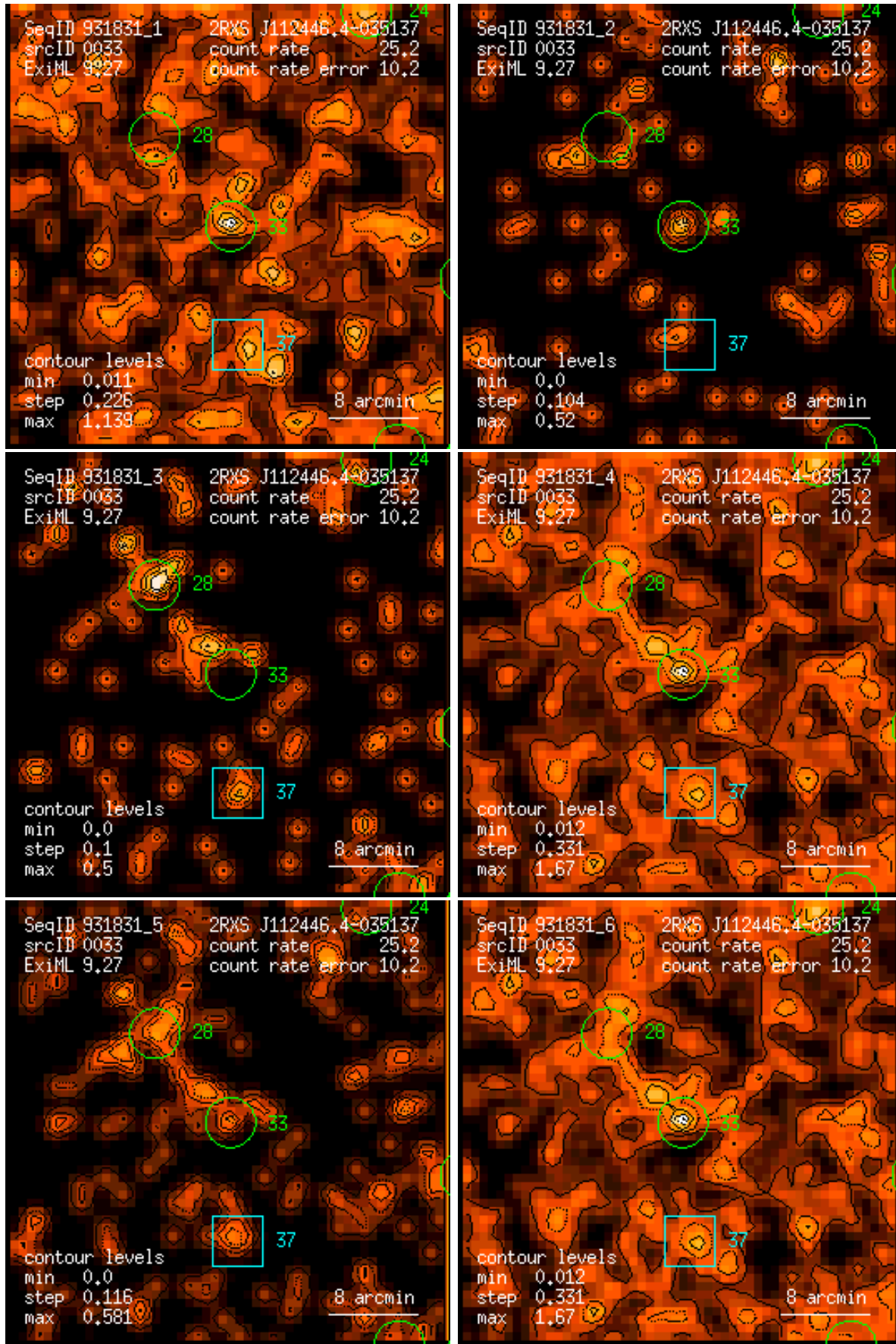
Figure 33: RASS 931831: detection 0033: band rate images, Gaussian filter: (1) PSPC channels 11 – 41, (2) 52 – 90, (3) 91 – 201, (4) 11 – 235, (5) 52 – 201, (6) 11 – 201. Broad band rates in counts/ks. Band rate contour levels in counts/ks/arcmin 2 .
