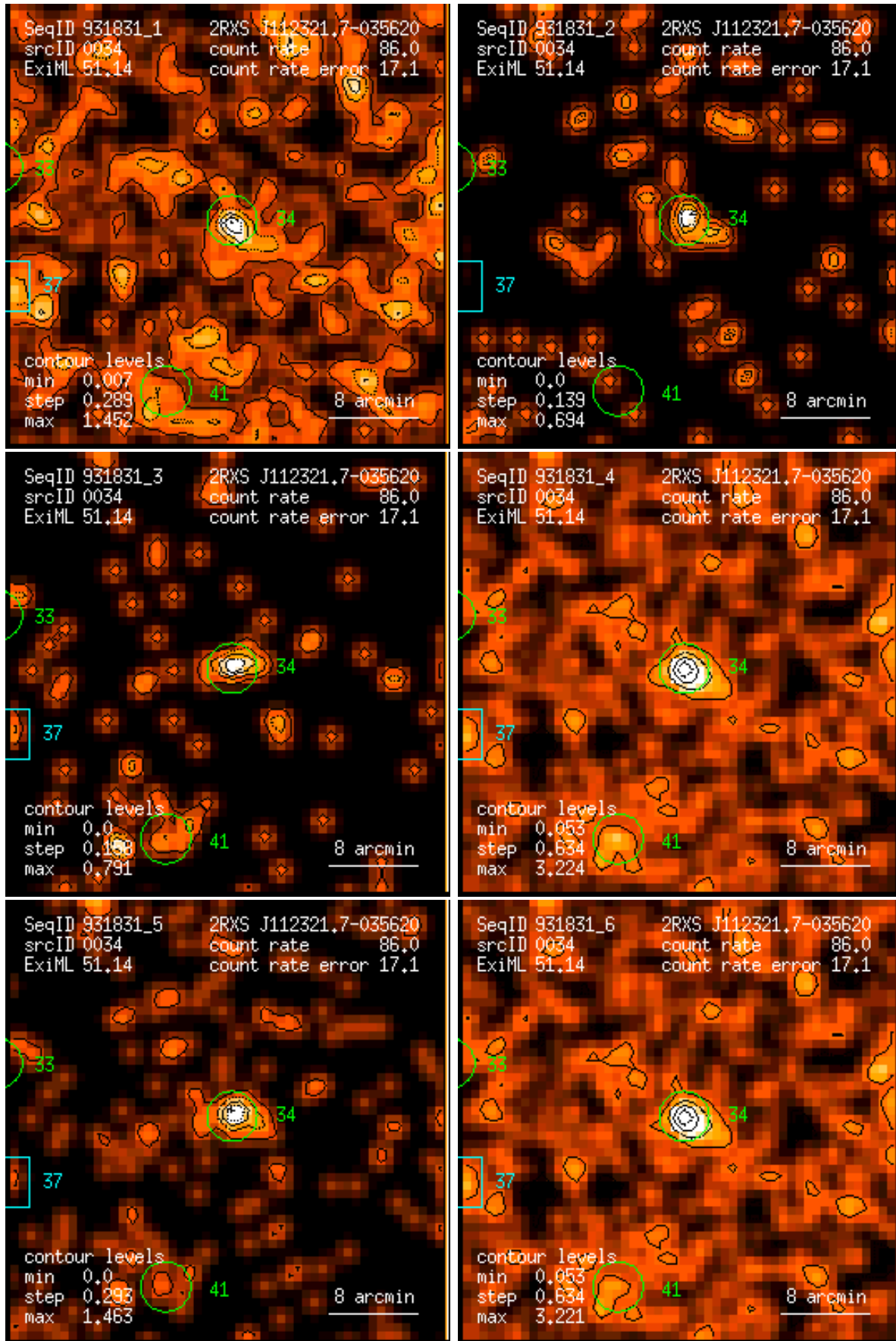
Figure 34: RASS 931831: detection 0034: band rate images, Gaussian filter: (1) PSPC channels 11 – 41, (2) 52 – 90, (3) 91 – 201, (4) 11 – 235, (5) 52 – 201, (6) 11 – 201. Broad band rates in counts/ks. Band rate contour levels in counts/ks/arcmin 2 .
