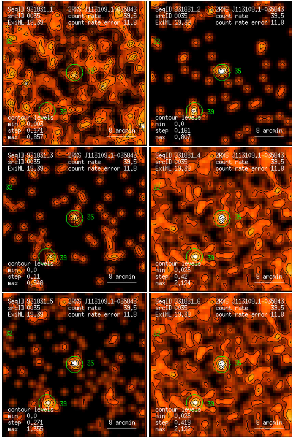
Figure 35: RASS 931831: detection 0035: band rate images, Gaussian filter: (1) PSPC channels 11 – 41, (2) 52 – 90, (3) 91 – 201, (4) 11 – 235, (5) 52 – 201, (6) 11 – 201. Broad band rates in counts/ks. Band rate contour levels in counts/ks/arcmin 2 .
