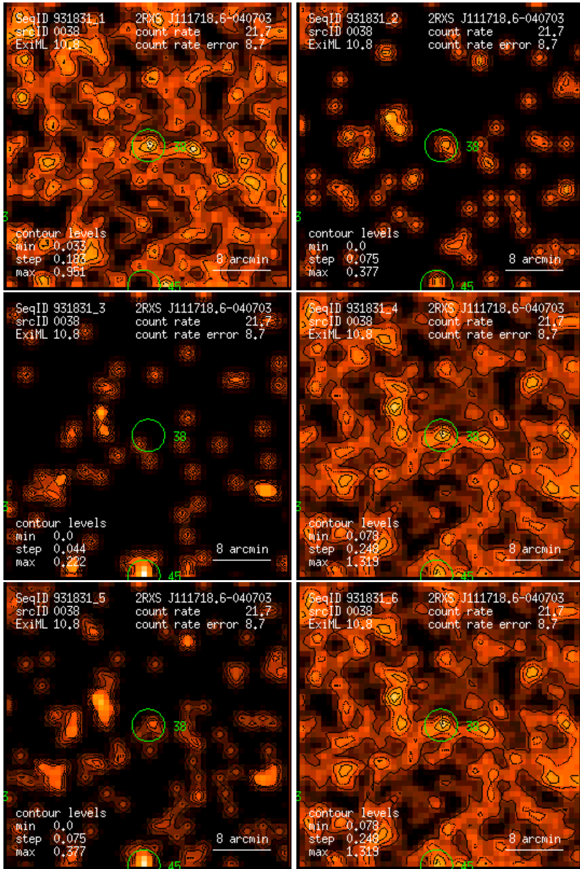
Figure 38: RASS 931831: detection 0038: band rate images, Gaussian filter: (1) PSPC channels 11 – 41, (2) 52 – 90, (3) 91 – 201, (4) 11 – 235, (5) 52 – 201, (6) 11 – 201. Broad band rates in counts/ks. Band rate contour levels in counts/ks/arcmin 2 .
