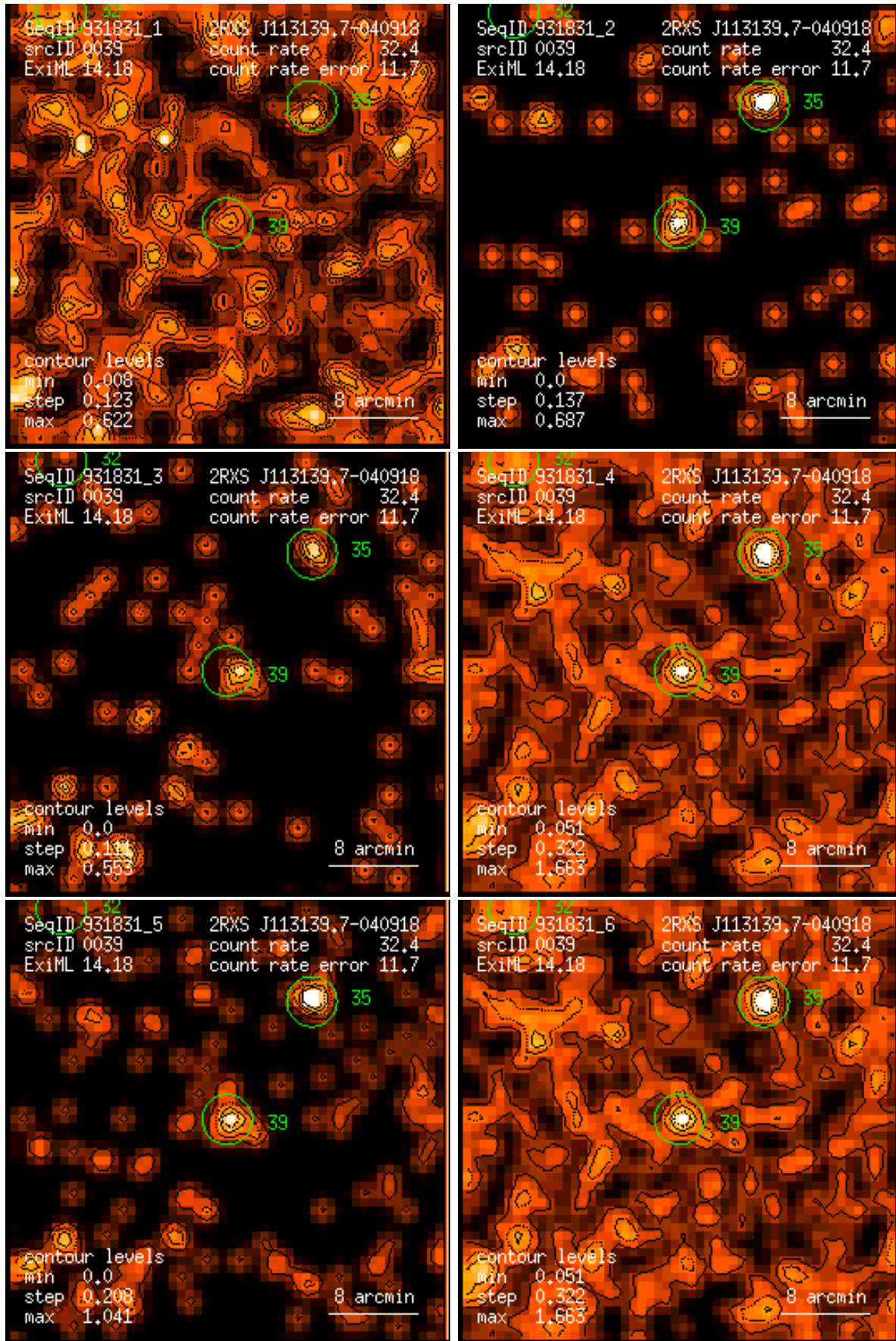
Figure 39: RASS 931831: detection 0039: band rate images, Gaussian filter: (1) PSPC channels 11 – 41, (2) 52 – 90, (3) 91 – 201, (4) 11 – 235, (5) 52 – 201, (6) 11 – 201. Broad band rates in counts/ks. Band rate contour levels in counts/ks/arcmin 2 .
