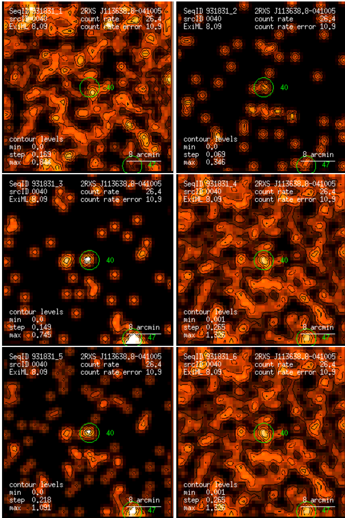
Figure 40: RASS 931831: detection 0040: band rate images, Gaussian filter: (1) PSPC channels 11 – 41, (2) 52 – 90, (3) 91 – 201, (4) 11 – 235, (5) 52 – 201, (6) 11 – 201. Broad band rates in counts/ks. Band rate contour levels in counts/ks/arcmin 2 .
