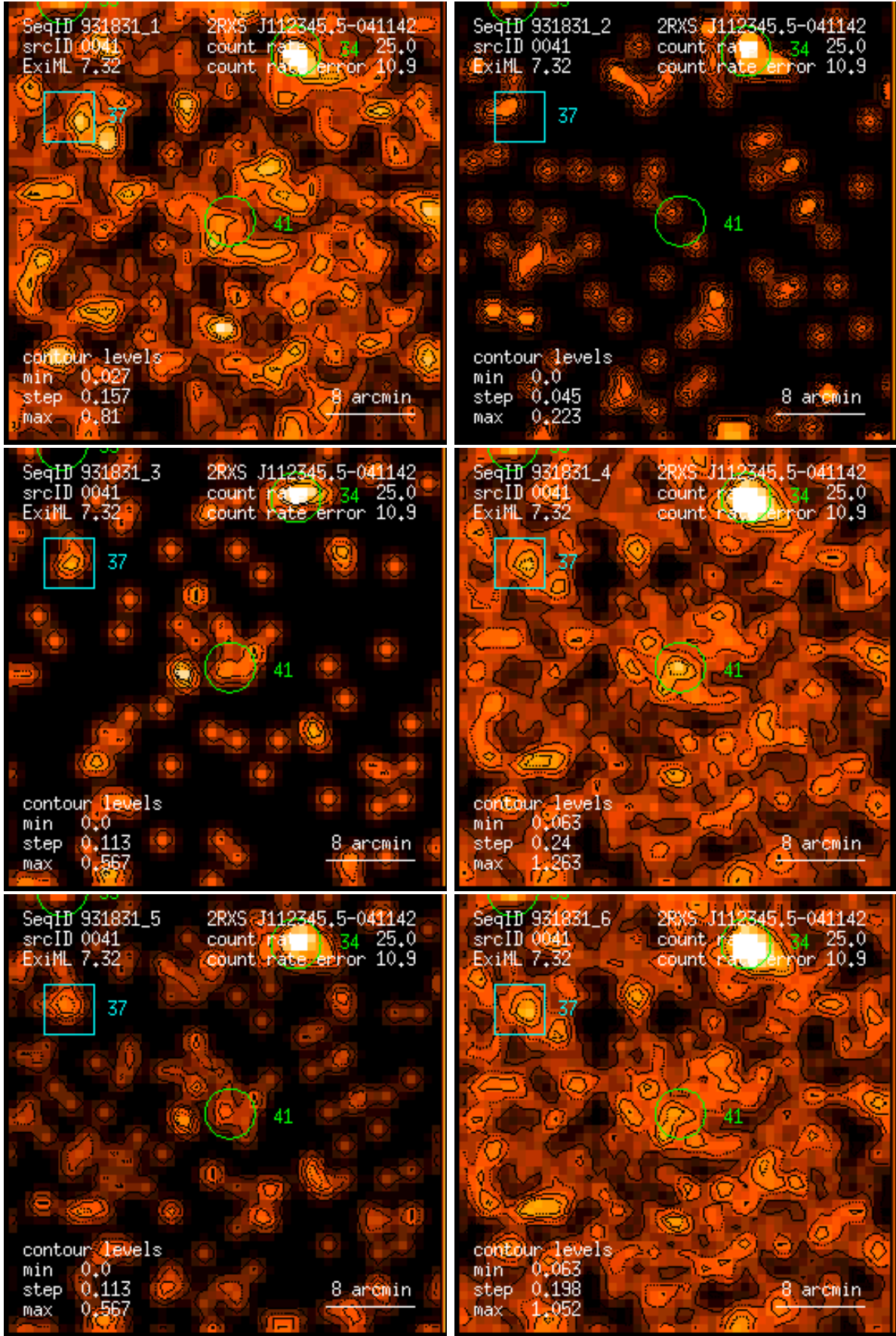
Figure 41: RASS 931831: detection 0041: band rate images, Gaussian filter: (1) PSPC channels 11 – 41, (2) 52 – 90, (3) 91 – 201, (4) 11 – 235, (5) 52 – 201, (6) 11 – 201. Broad band rates in counts/ks. Band rate contour levels in counts/ks/arcmin 2 .
