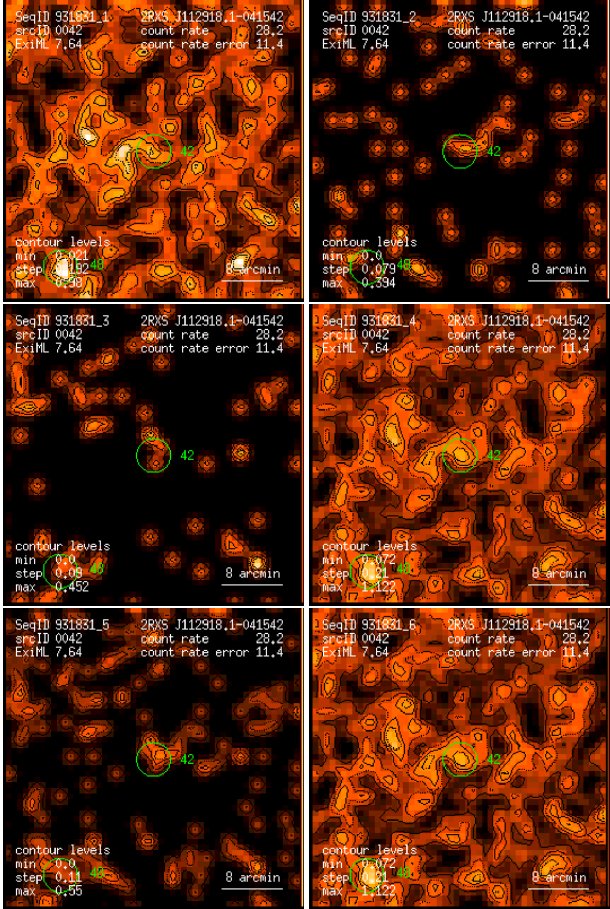
Figure 42: RASS 931831: detection 0042: band rate images, Gaussian filter: (1) PSPC channels 11 – 41, (2) 52 – 90, (3) 91 – 201, (4) 11 – 235, (5) 52 – 201, (6) 11 – 201. Broad band rates in counts/ks. Band rate contour levels in counts/ks/arcmin 2 .
