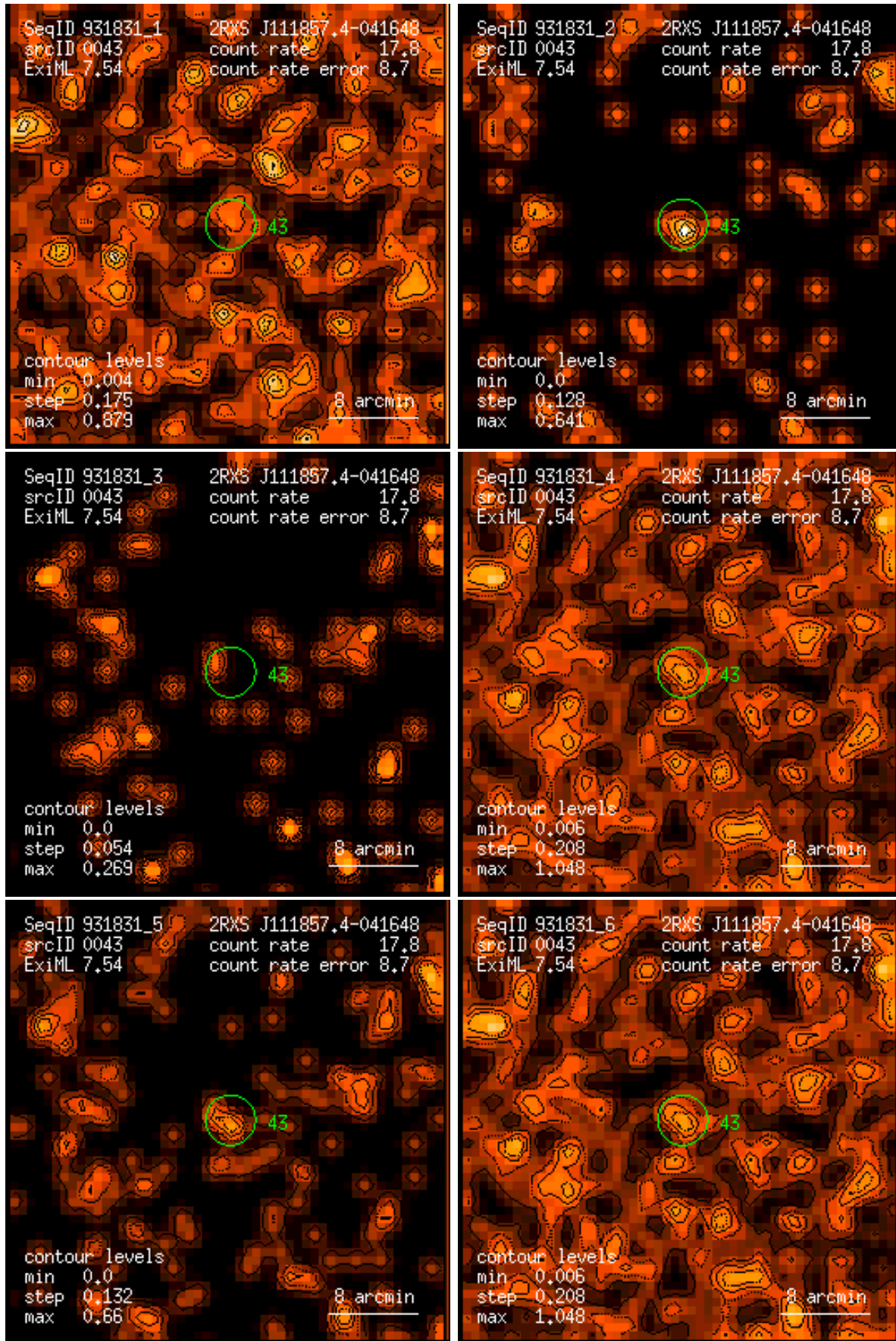
Figure 43: RASS 931831: detection 0043: band rate images, Gaussian filter: (1) PSPC channels 11 – 41, (2) 52 – 90, (3) 91 – 201, (4) 11 – 235, (5) 52 – 201, (6) 11 – 201. Broad band rates in counts/ks. Band rate contour levels in counts/ks/arcmin 2 .
