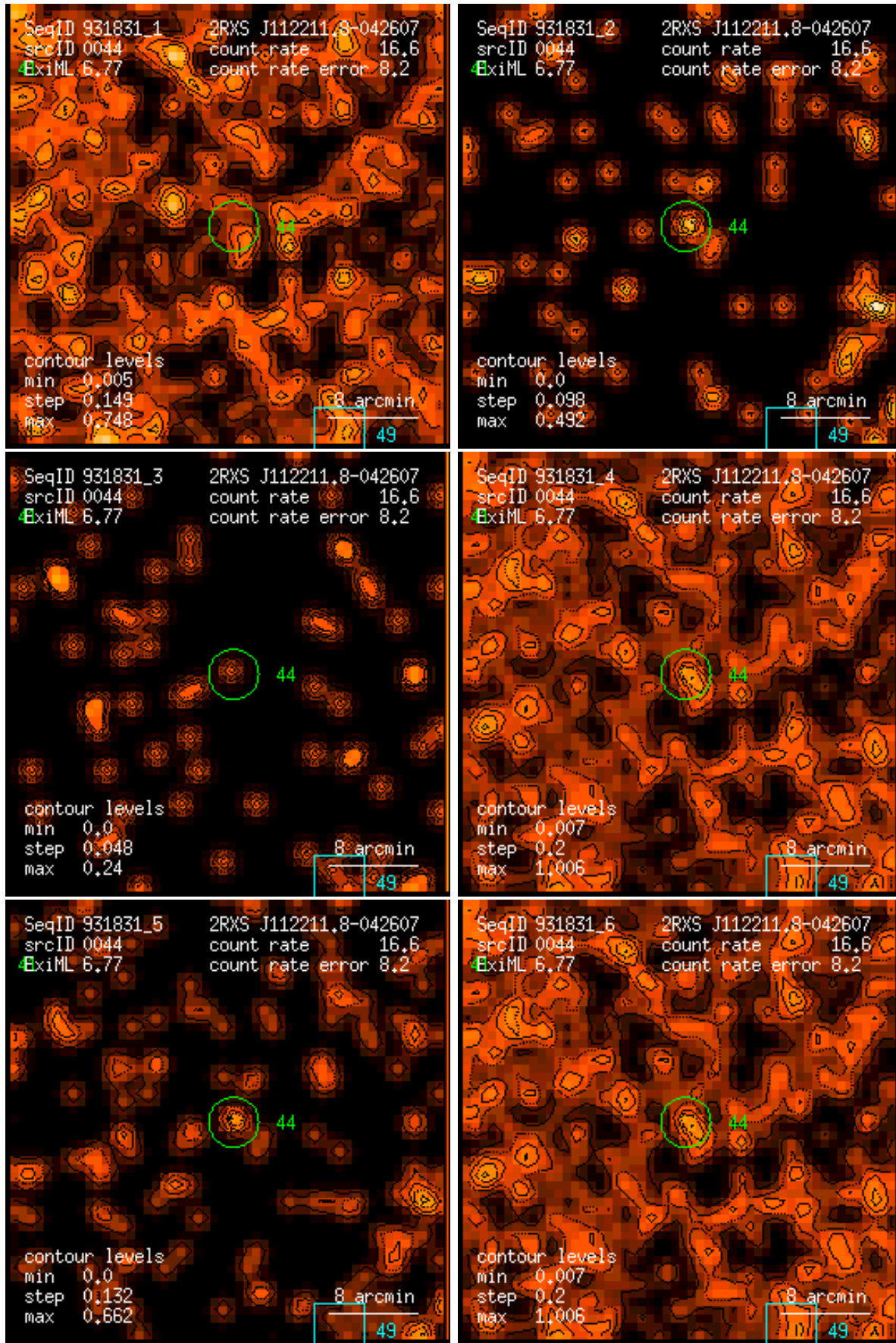
Figure 44: RASS 931831: detection 0044: band rate images, Gaussian filter: (1) PSPC channels 11 – 41, (2) 52 – 90, (3) 91 – 201, (4) 11 – 235, (5) 52 – 201, (6) 11 – 201. Broad band rates in counts/ks. Band rate contour levels in counts/ks/arcmin 2 .
