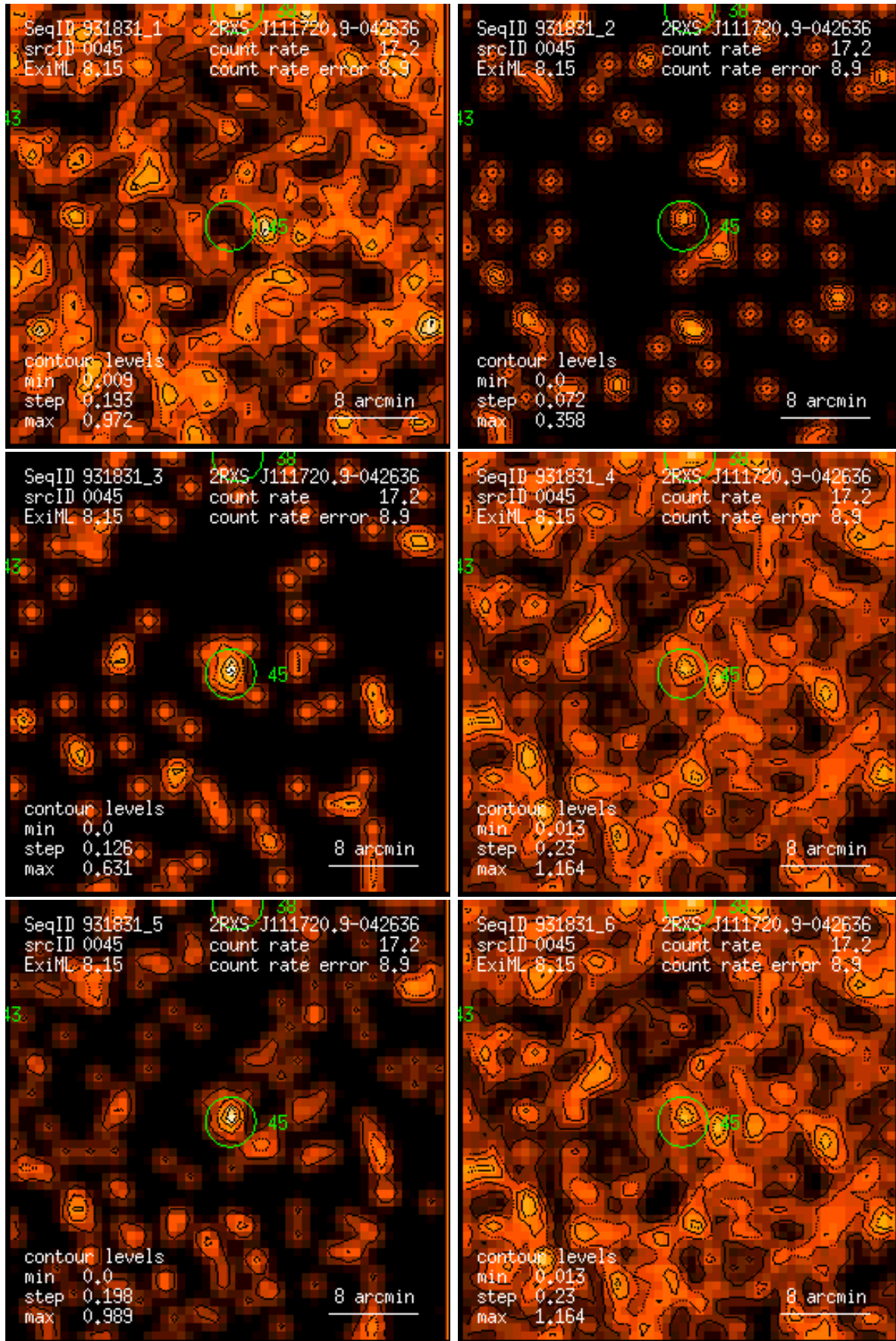
Figure 45: RASS 931831: detection 0045: band rate images, Gaussian filter: (1) PSPC channels 11 – 41, (2) 52 – 90, (3) 91 – 201, (4) 11 – 235, (5) 52 – 201, (6) 11 – 201. Broad band rates in counts/ks. Band rate contour levels in counts/ks/arcmin 2 .
