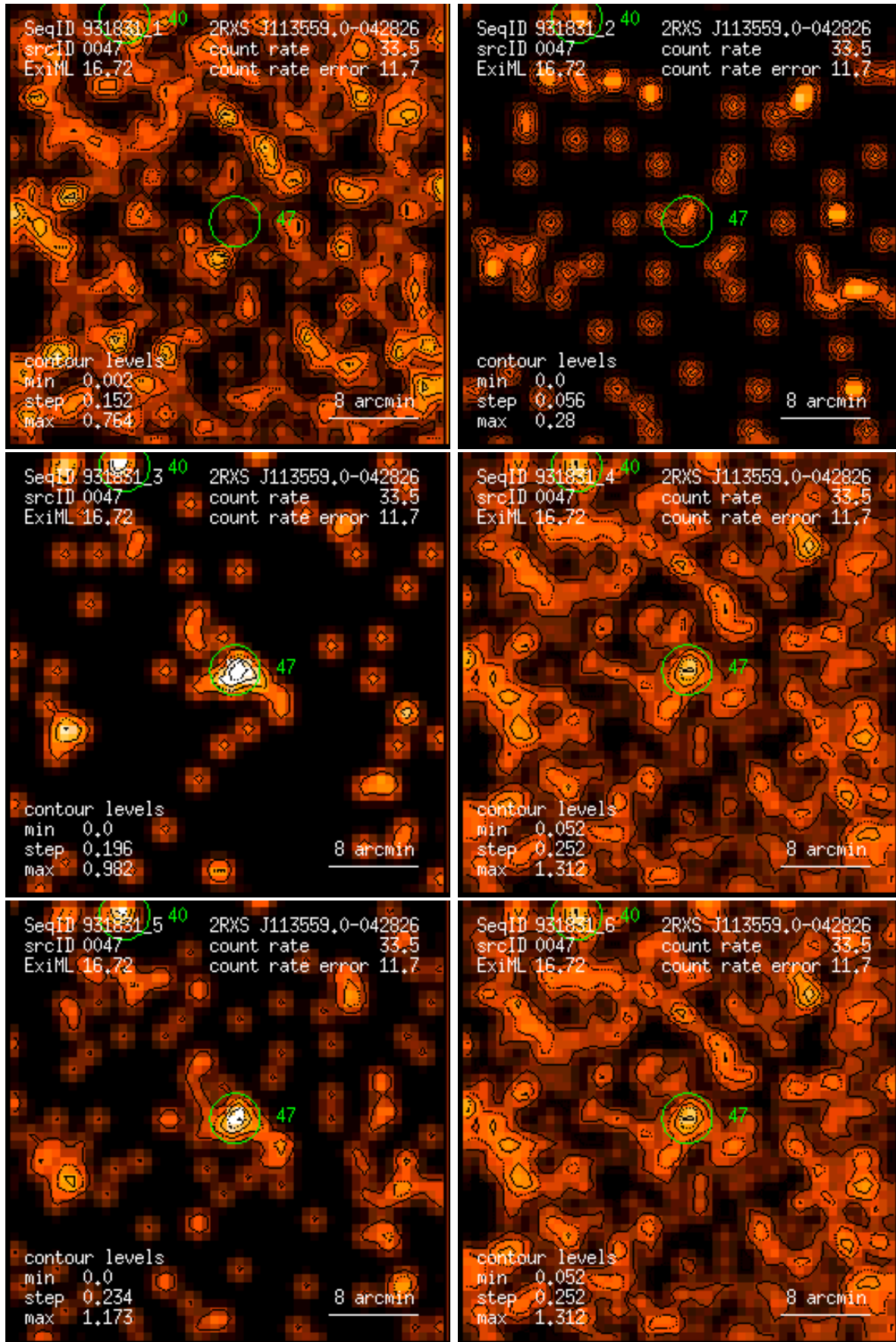
Figure 47: RASS 931831: detection 0047: band rate images, Gaussian filter: (1) PSPC channels 11 – 41, (2) 52 – 90, (3) 91 – 201, (4) 11 – 235, (5) 52 – 201, (6) 11 – 201. Broad band rates in counts/ks. Band rate contour levels in counts/ks/arcmin 2 .
