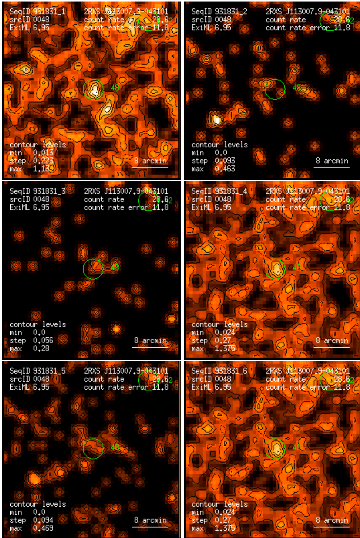
Figure 48: RASS 931831: detection 0048: band rate images, Gaussian filter: (1) PSPC channels 11 – 41, (2) 52 – 90, (3) 91 – 201, (4) 11 – 235, (5) 52 – 201, (6) 11 – 201. Broad band rates in counts/ks. Band rate contour levels in counts/ks/arcmin 2 .
