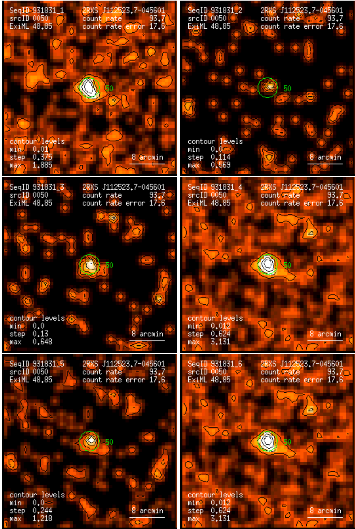
Figure 50: RASS 931831: detection 0050: band rate images, Gaussian filter: (1) PSPC channels 11 – 41, (2) 52 – 90, (3) 91 – 201, (4) 11 – 235, (5) 52 – 201, (6) 11 – 201. Broad band rates in counts/ks. Band rate contour levels in counts/ks/arcmin 2 .
