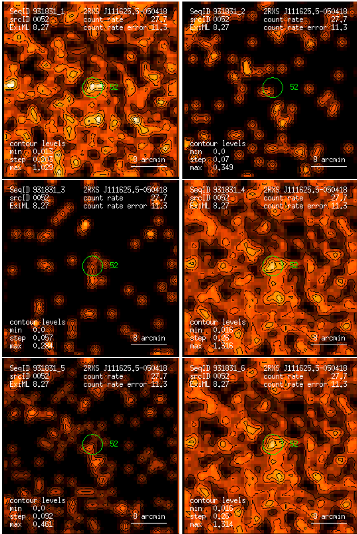
Figure 52: RASS 931831: detection 0052: band rate images, Gaussian filter: (1) PSPC channels 11 – 41, (2) 52 – 90, (3) 91 – 201, (4) 11 – 235, (5) 52 – 201, (6) 11 – 201. Broad band rates in counts/ks. Band rate contour levels in counts/ks/arcmin 2 .
