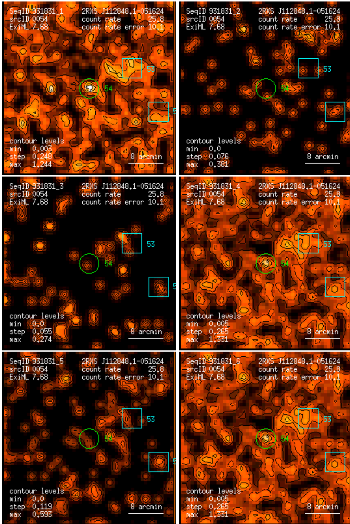
Figure 54: RASS 931831: detection 0054: band rate images, Gaussian filter: (1) PSPC channels 11 – 41, (2) 52 – 90, (3) 91 – 201, (4) 11 – 235, (5) 52 – 201, (6) 11 – 201. Broad band rates in counts/ks. Band rate contour levels in counts/ks/arcmin 2 .
