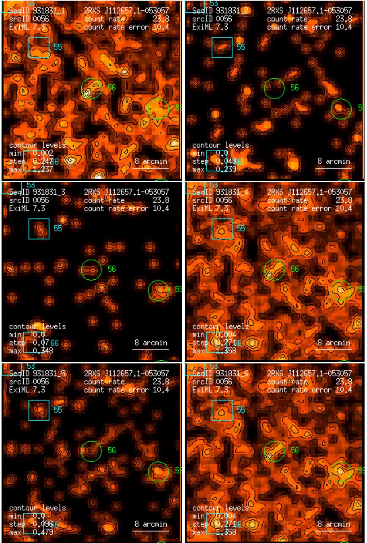
Figure 56: RASS 931831: detection 0056: band rate images, Gaussian filter: (1) PSPC channels 11 – 41, (2) 52 – 90, (3) 91 – 201, (4) 11 – 235, (5) 52 – 201, (6) 11 – 201. Broad band rates in counts/ks. Band rate contour levels in counts/ks/arcmin 2 .
