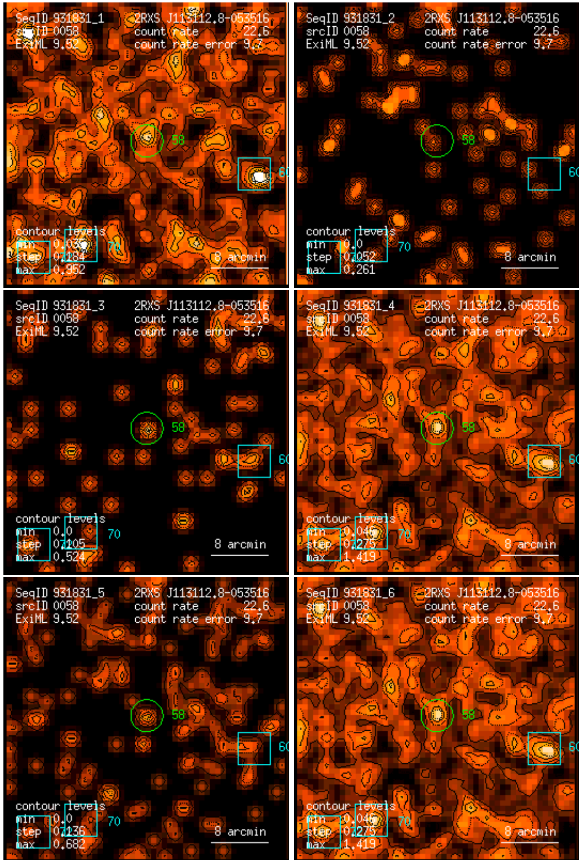
Figure 58: RASS 931831: detection 0058: band rate images, Gaussian filter: (1) PSPC channels 11 – 41, (2) 52 – 90, (3) 91 – 201, (4) 11 – 235, (5) 52 – 201, (6) 11 – 201. Broad band rates in counts/ks. Band rate contour levels in counts/ks/arcmin 2 .
