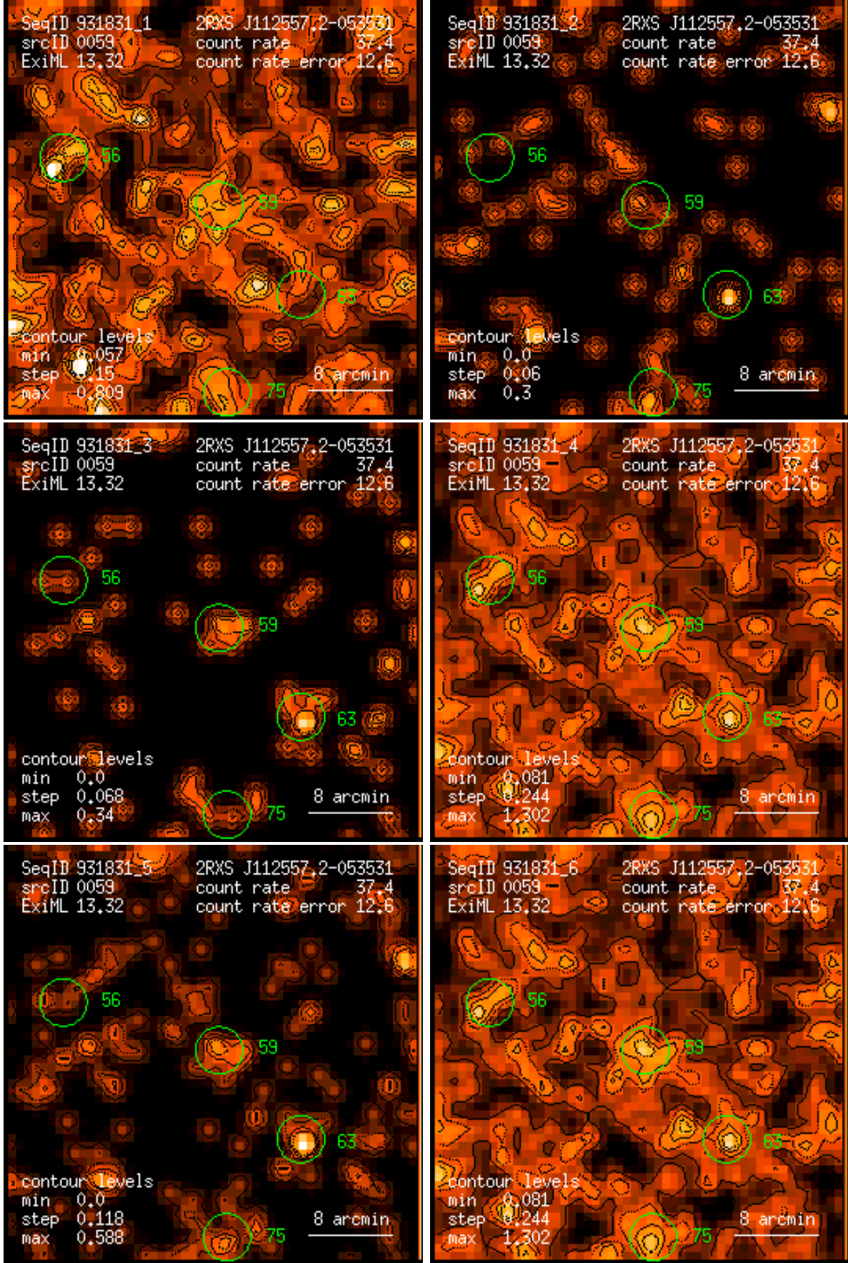
Figure 59: RASS 931831: detection 0059: band rate images, Gaussian filter: (1) PSPC channels 11 – 41, (2) 52 – 90, (3) 91 – 201, (4) 11 – 235, (5) 52 – 201, (6) 11 – 201. Broad band rates in counts/ks. Band rate contour levels in counts/ks/arcmin 2 .
