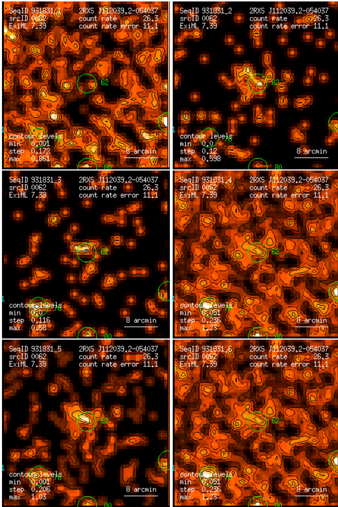
Figure 62: RASS 931831: detection 0062: band rate images, Gaussian filter: (1) PSPC channels 11 – 41, (2) 52 – 90, (3) 91 – 201, (4) 11 – 235, (5) 52 – 201, (6) 11 – 201. Broad band rates in counts/ks. Band rate contour levels in counts/ks/arcmin 2 .
