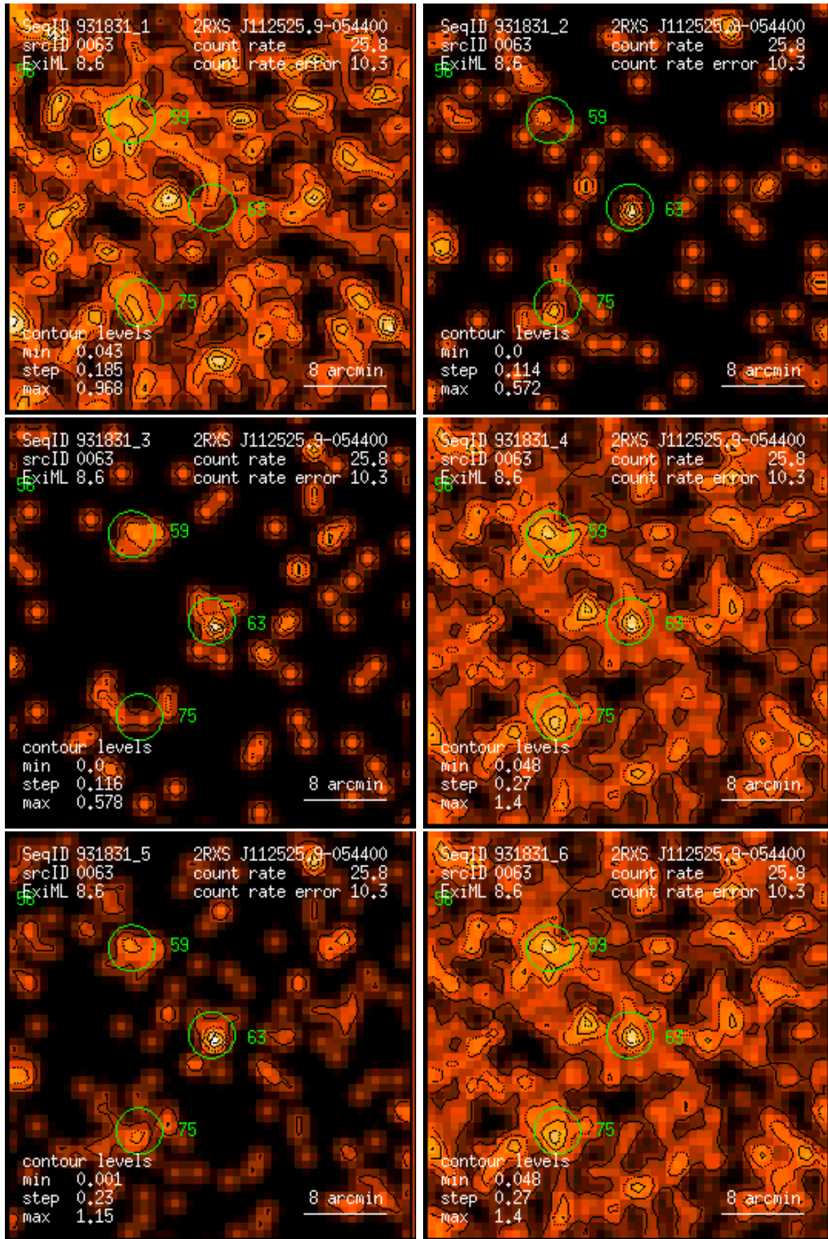
Figure 63: RASS 931831: detection 0063: band rate images, Gaussian filter: (1) PSPC channels 11 – 41, (2) 52 – 90, (3) 91 – 201, (4) 11 – 235, (5) 52 – 201, (6) 11 – 201. Broad band rates in counts/ks. Band rate contour levels in counts/ks/arcmin 2 .
