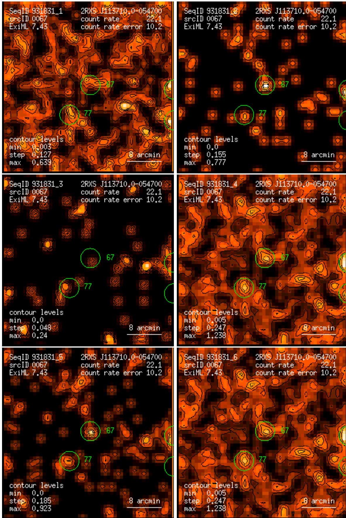
Figure 67: RASS 931831: detection 0067: band rate images, Gaussian filter: (1) PSPC channels 11 – 41, (2) 52 – 90, (3) 91 – 201, (4) 11 – 235, (5) 52 – 201, (6) 11 – 201. Broad band rates in counts/ks. Band rate contour levels in counts/ks/arcmin 2 .
