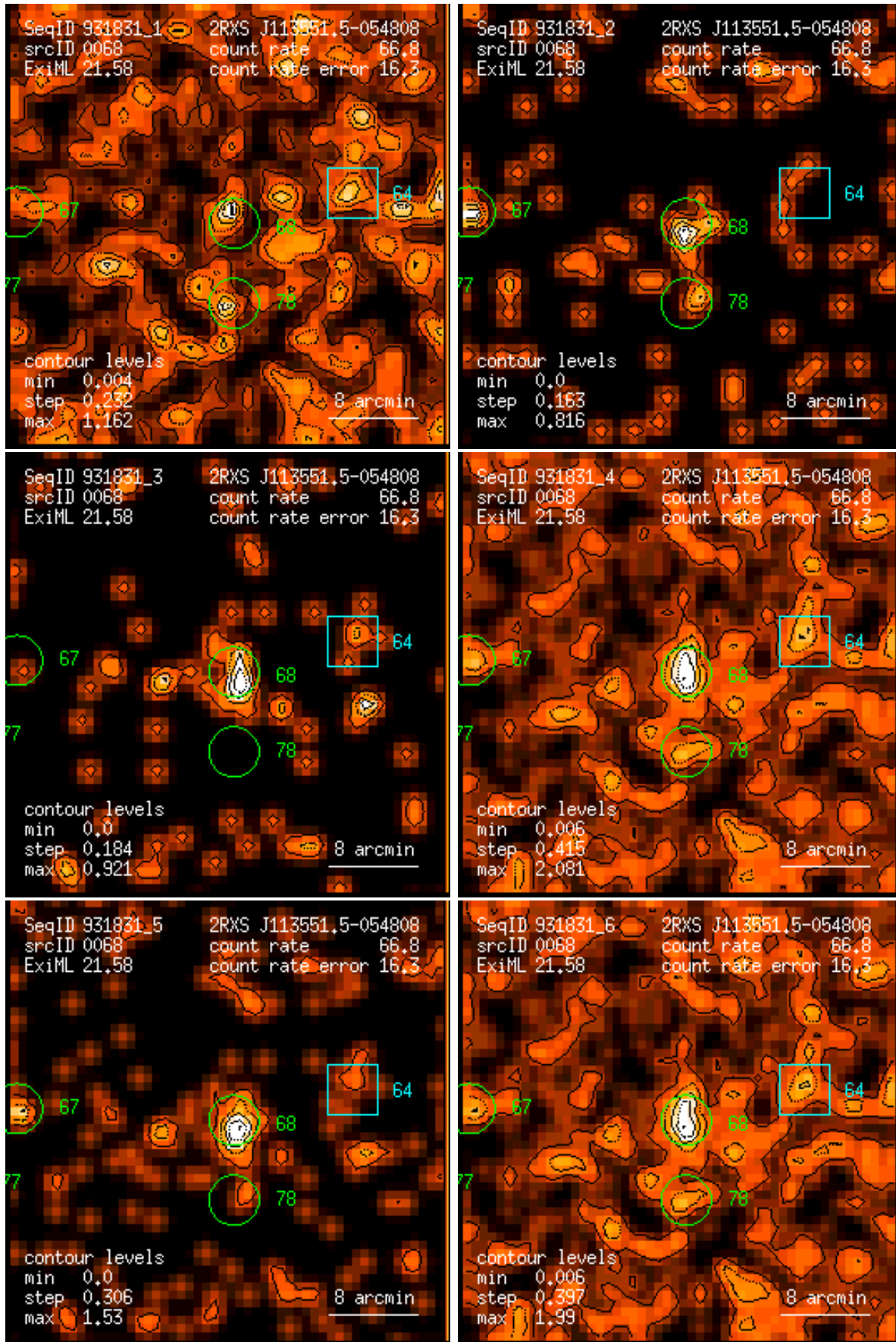
Figure 68: RASS 931831: detection 0068: band rate images, Gaussian filter: (1) PSPC channels 11 – 41, (2) 52 – 90, (3) 91 – 201, (4) 11 – 235, (5) 52 – 201, (6) 11 – 201. Broad band rates in counts/ks. Band rate contour levels in counts/ks/arcmin 2 .
