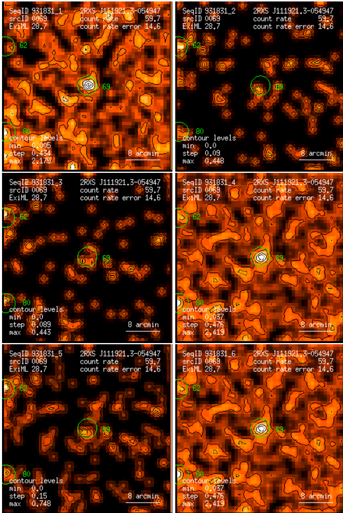
Figure 69: RASS 931831: detection 0069: band rate images, Gaussian filter: (1) PSPC channels 11 – 41, (2) 52 – 90, (3) 91 – 201, (4) 11 – 235, (5) 52 – 201, (6) 11 – 201. Broad band rates in counts/ks. Band rate contour levels in counts/ks/arcmin 2 .
