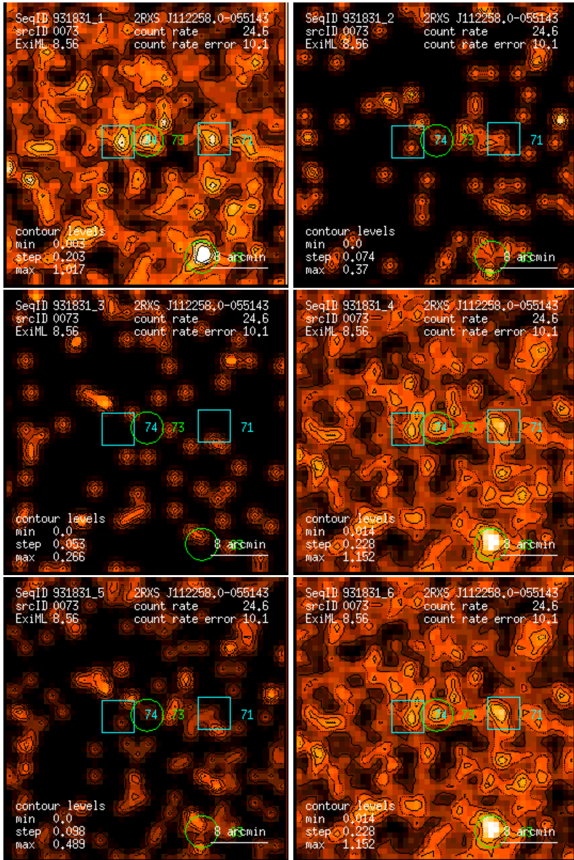
Figure 73: RASS 931831: detection 0073: band rate images, Gaussian filter: (1) PSPC channels 11 – 41, (2) 52 – 90, (3) 91 – 201, (4) 11 – 235, (5) 52 – 201, (6) 11 – 201. Broad band rates in counts/ks. Band rate contour levels in counts/ks/arcmin 2 .
