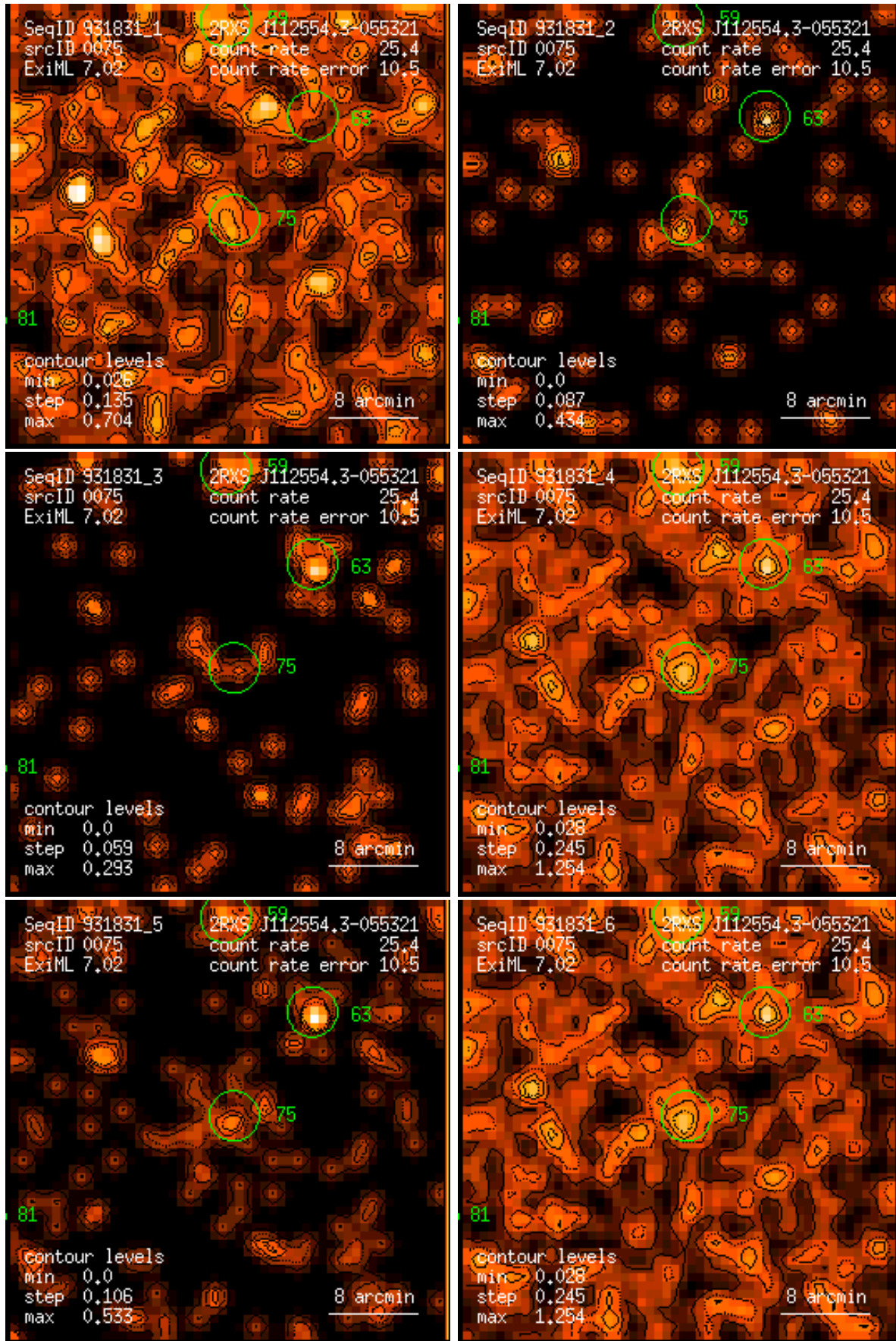
Figure 75: RASS 931831: detection 0075: band rate images, Gaussian filter: (1) PSPC channels 11 – 41, (2) 52 – 90, (3) 91 – 201, (4) 11 – 235, (5) 52 – 201, (6) 11 – 201. Broad band rates in counts/ks. Band rate contour levels in counts/ks/arcmin 2 .
