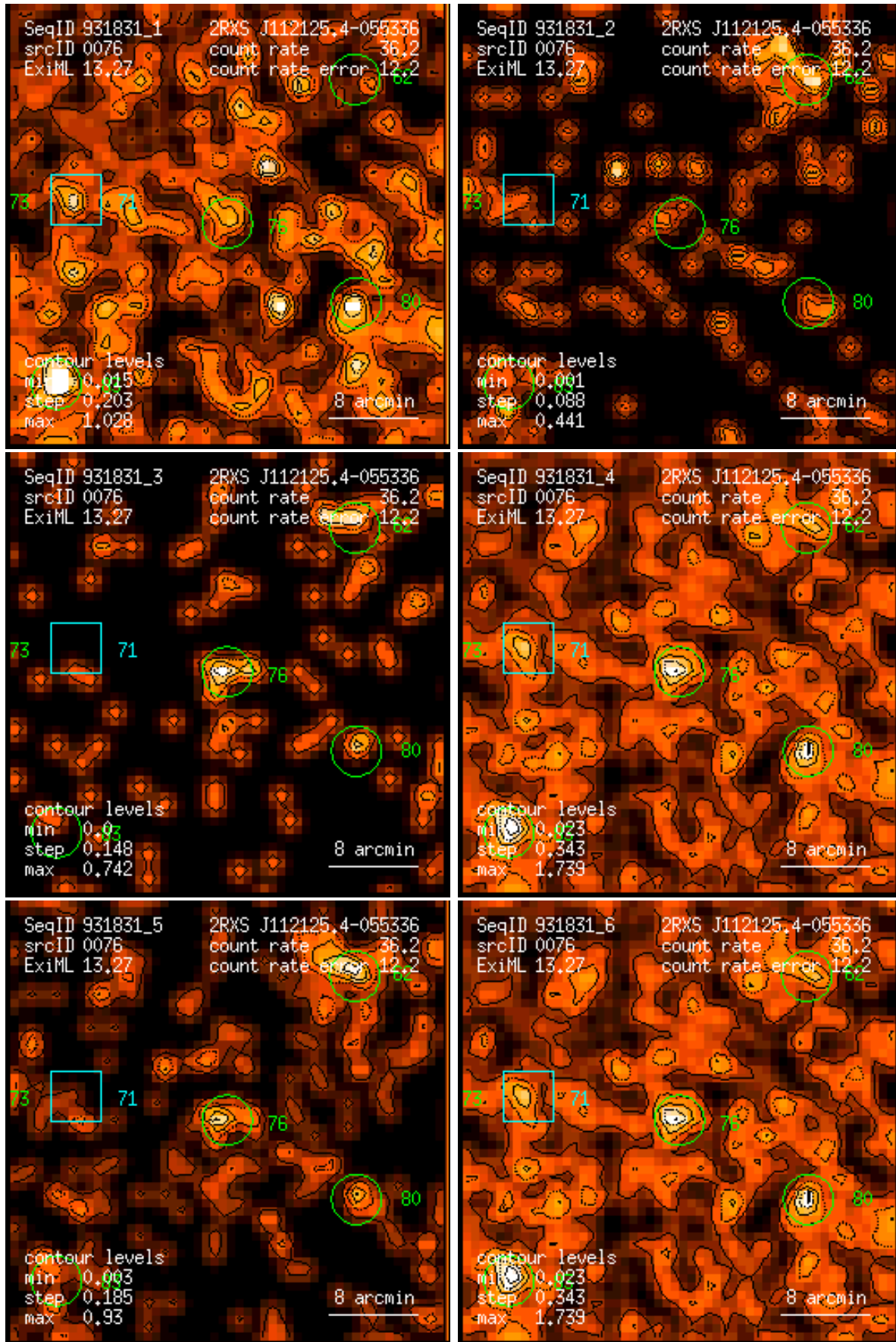
Figure 76: RASS 931831: detection 0076: band rate images, Gaussian filter: (1) PSPC channels 11 – 41, (2) 52 – 90, (3) 91 – 201, (4) 11 – 235, (5) 52 – 201, (6) 11 – 201. Broad band rates in counts/ks. Band rate contour levels in counts/ks/arcmin 2 .
