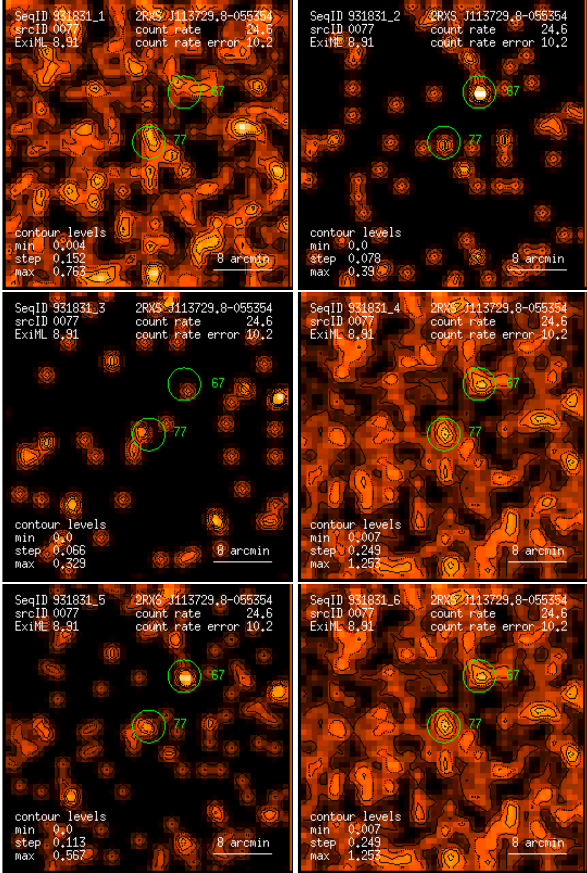
Figure 77: RASS 931831: detection 0077: band rate images, Gaussian filter: (1) PSPC channels 11 – 41, (2) 52 – 90, (3) 91 – 201, (4) 11 – 235, (5) 52 – 201, (6) 11 – 201. Broad band rates in counts/ks. Band rate contour levels in counts/ks/arcmin 2 .
