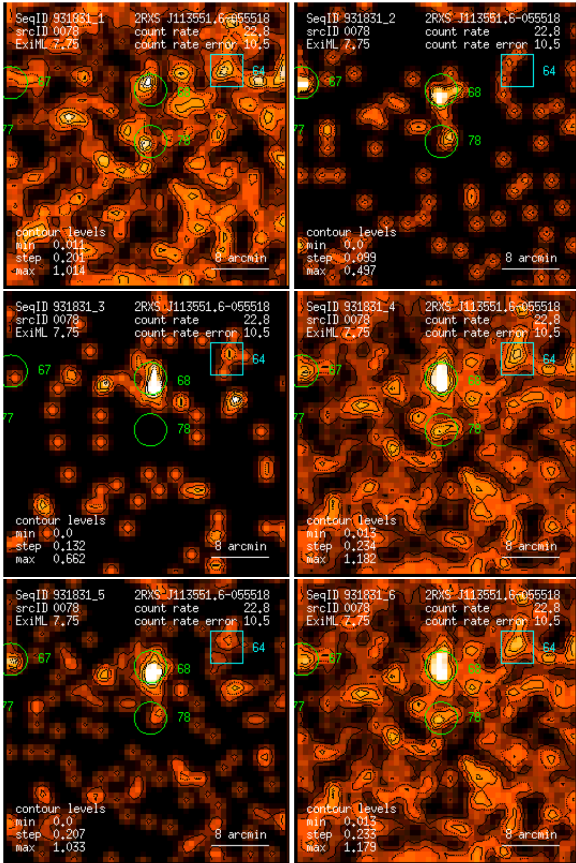
Figure 78: RASS 931831: detection 0078: band rate images, Gaussian filter: (1) PSPC channels 11 – 41, (2) 52 – 90, (3) 91 – 201, (4) 11 – 235, (5) 52 – 201, (6) 11 – 201. Broad band rates in counts/ks. Band rate contour levels in counts/ks/arcmin 2 .
