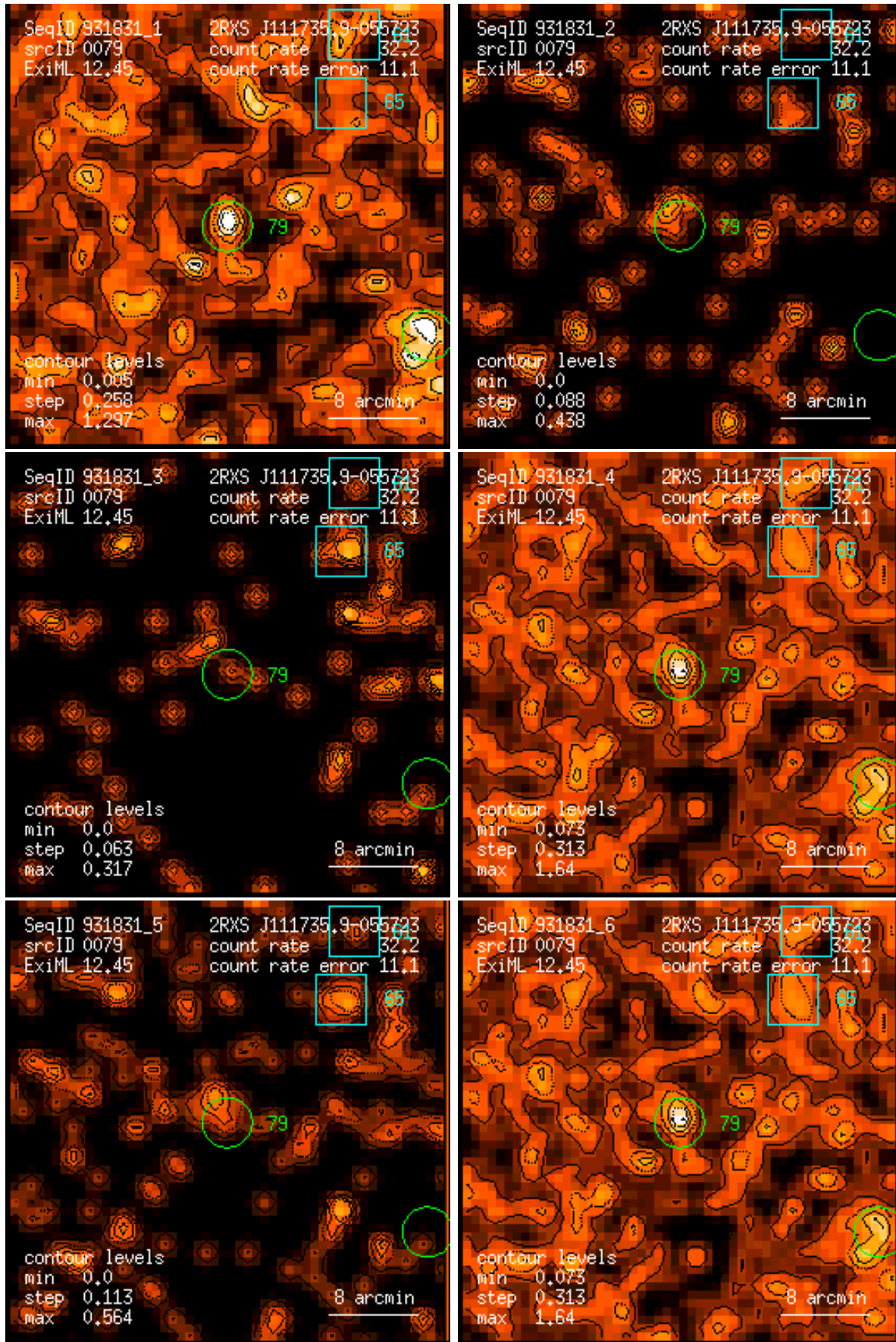
Figure 79: RASS 931831: detection 0079: band rate images, Gaussian filter: (1) PSPC channels 11 – 41, (2) 52 – 90, (3) 91 – 201, (4) 11 – 235, (5) 52 – 201, (6) 11 – 201. Broad band rates in counts/ks. Band rate contour levels in counts/ks/arcmin 2 .
