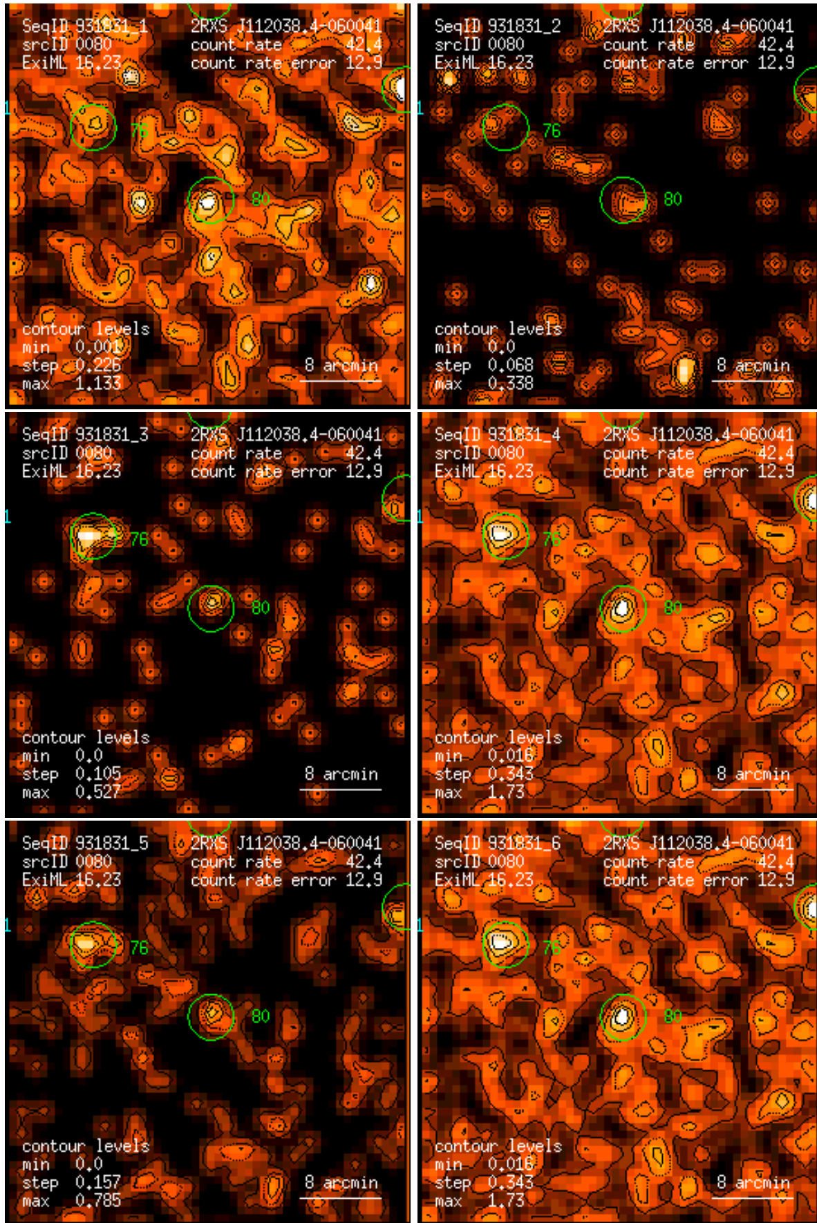
Figure 80: RASS 931831: detection 0080: band rate images, Gaussian filter: (1) PSPC channels 11 – 41, (2) 52 – 90, (3) 91 – 201, (4) 11 – 235, (5) 52 – 201, (6) 11 – 201. Broad band rates in counts/ks. Band rate contour levels in counts/ks/arcmin 2 .
