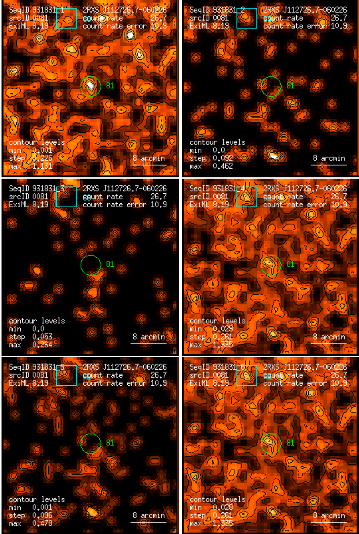
Figure 81: RASS 931831: detection 0081: band rate images, Gaussian filter: (1) PSPC channels 11 – 41, (2) 52 – 90, (3) 91 – 201, (4) 11 – 235, (5) 52 – 201, (6) 11 – 201. Broad band rates in counts/ks. Band rate contour levels in counts/ks/arcmin 2 .
