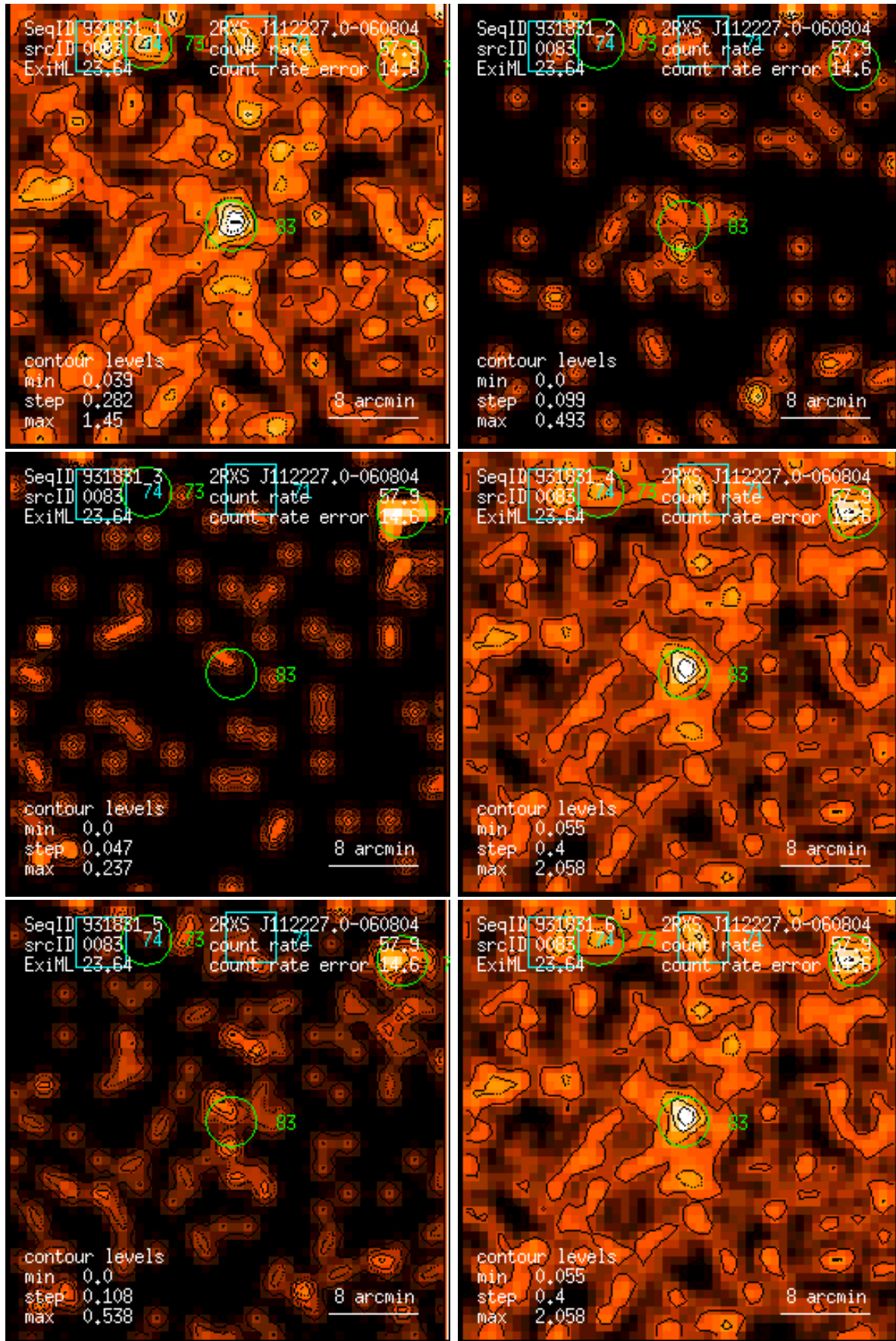
Figure 83: RASS 931831: detection 0083: band rate images, Gaussian filter: (1) PSPC channels 11 – 41, (2) 52 – 90, (3) 91 – 201, (4) 11 – 235, (5) 52 – 201, (6) 11 – 201. Broad band rates in counts/ks. Band rate contour levels in counts/ks/arcmin 2 .
