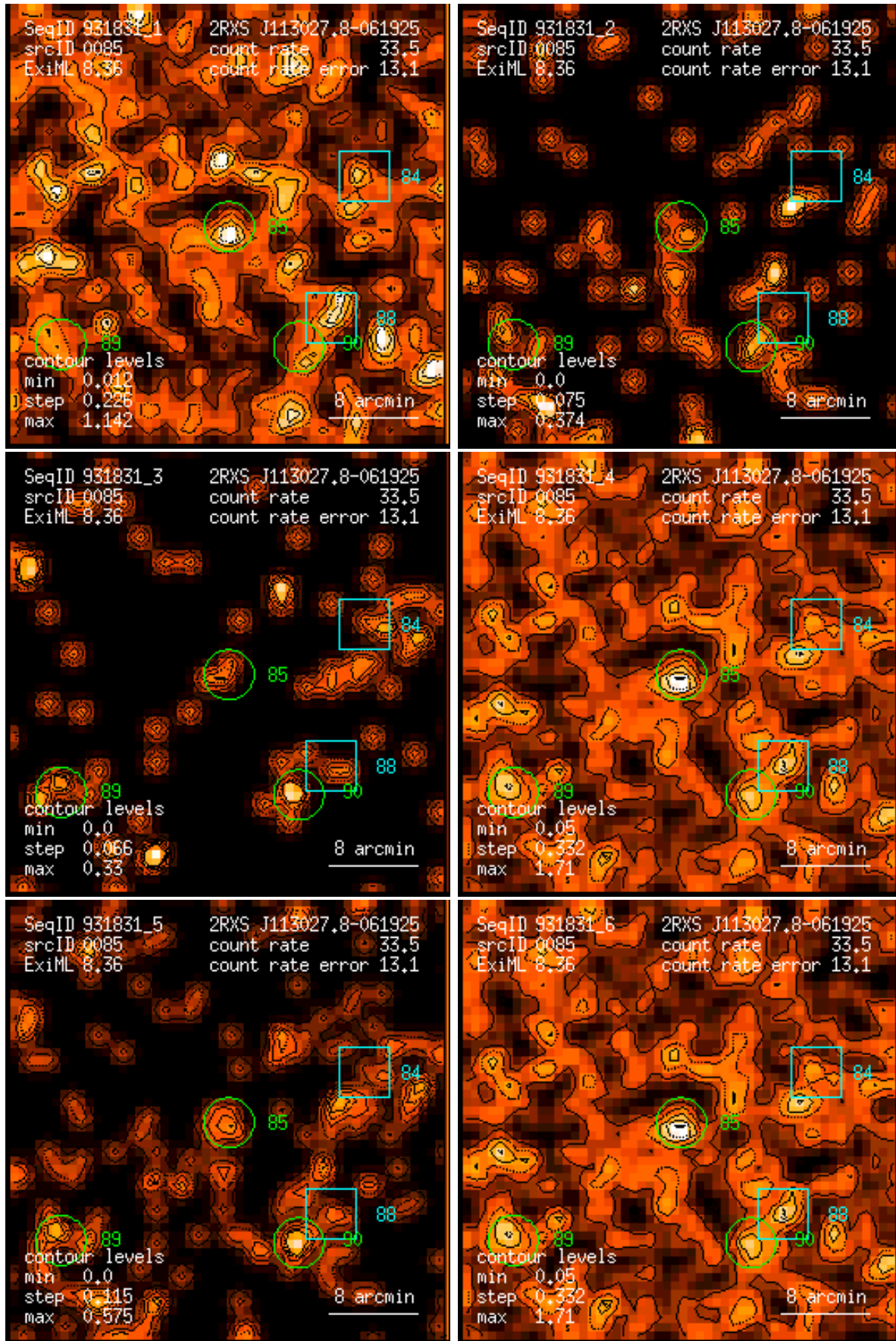
Figure 85: RASS 931831: detection 0085: band rate images, Gaussian filter: (1) PSPC channels 11 – 41, (2) 52 – 90, (3) 91 – 201, (4) 11 – 235, (5) 52 – 201, (6) 11 – 201. Broad band rates in counts/ks. Band rate contour levels in counts/ks/arcmin 2 .
