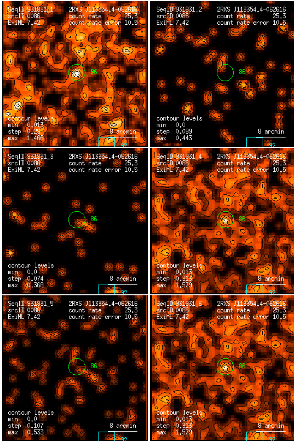
Figure 86: RASS 931831: detection 0086: band rate images, Gaussian filter: (1) PSPC channels 11 – 41, (2) 52 – 90, (3) 91 – 201, (4) 11 – 235, (5) 52 – 201, (6) 11 – 201. Broad band rates in counts/ks. Band rate contour levels in counts/ks/arcmin 2 .
