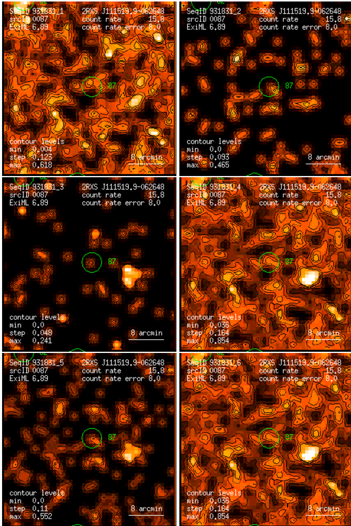
Figure 87: RASS 931831: detection 0087: band rate images, Gaussian filter: (1) PSPC channels 11 – 41, (2) 52 – 90, (3) 91 – 201, (4) 11 – 235, (5) 52 – 201, (6) 11 – 201. Broad band rates in counts/ks. Band rate contour levels in counts/ks/arcmin 2 .
