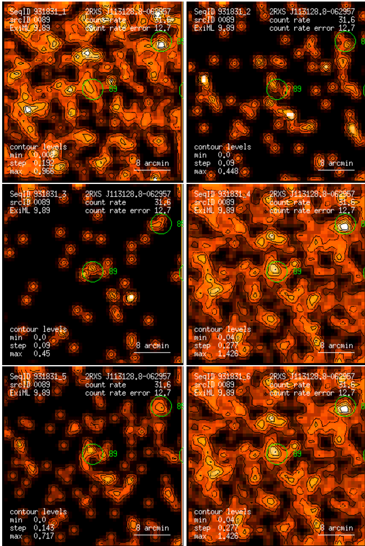
Figure 89: RASS 931831: detection 0089: band rate images, Gaussian filter: (1) PSPC channels 11 – 41, (2) 52 – 90, (3) 91 – 201, (4) 11 – 235, (5) 52 – 201, (6) 11 – 201. Broad band rates in counts/ks. Band rate contour levels in counts/ks/arcmin 2 .
