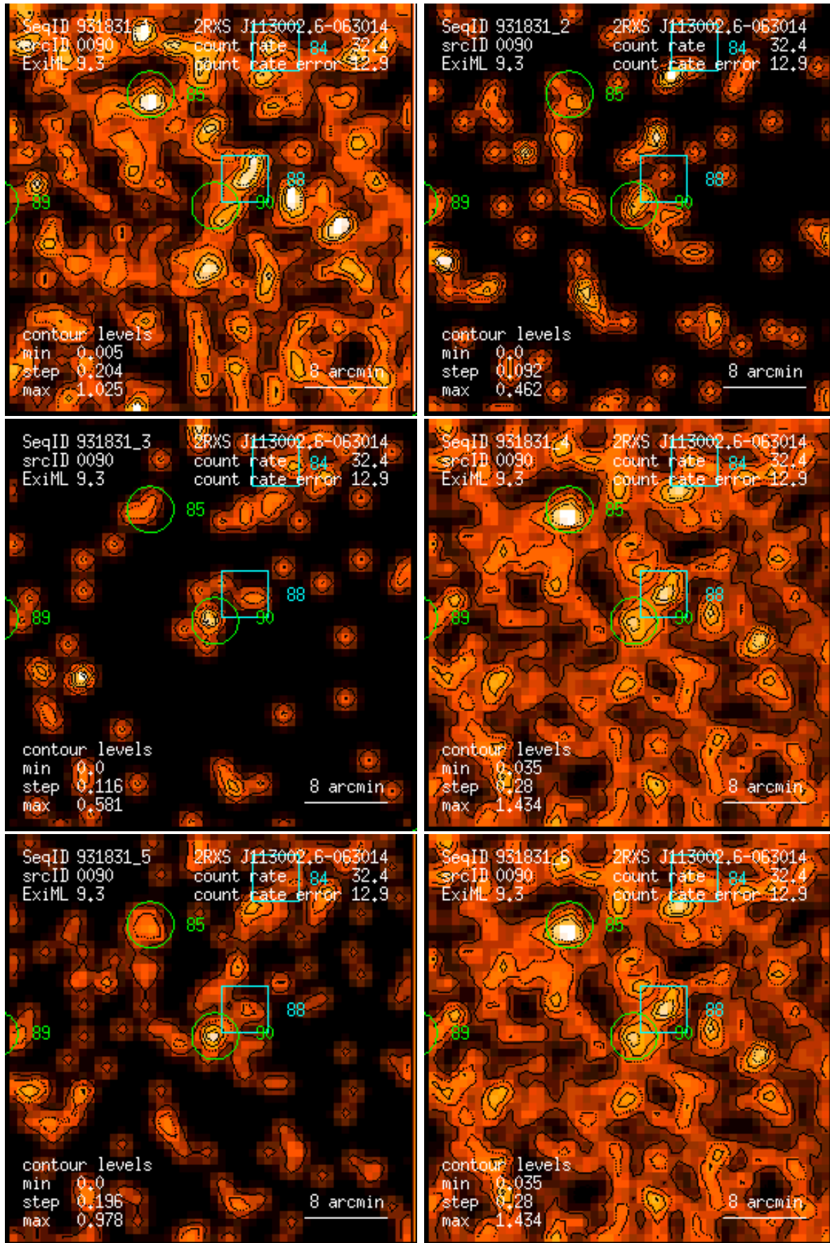
Figure 90: RASS 931831: detection 0090: band rate images, Gaussian filter: (1) PSPC channels 11 – 41, (2) 52 – 90, (3) 91 – 201, (4) 11 – 235, (5) 52 – 201, (6) 11 – 201. Broad band rates in counts/ks. Band rate contour levels in counts/ks/arcmin 2 .
