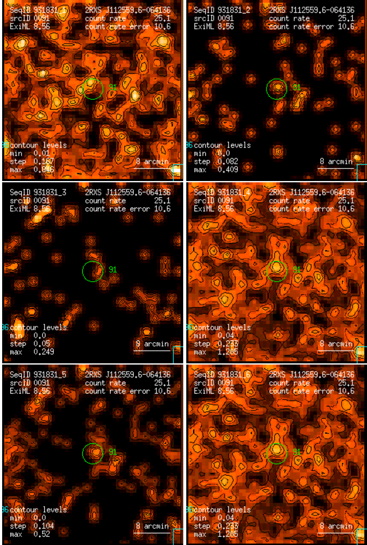
Figure 91: RASS 931831: detection 0091: band rate images, Gaussian filter: (1) PSPC channels 11 – 41, (2) 52 – 90, (3) 91 – 201, (4) 11 – 235, (5) 52 – 201, (6) 11 – 201. Broad band rates in counts/ks. Band rate contour levels in counts/ks/arcmin 2 .
