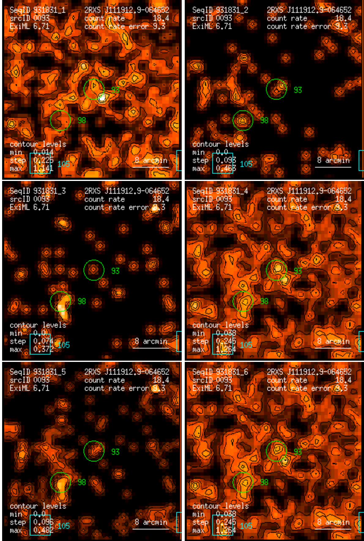
Figure 93: RASS 931831: detection 0093: band rate images, Gaussian filter: (1) PSPC channels 11 – 41, (2) 52 – 90, (3) 91 – 201, (4) 11 – 235, (5) 52 – 201, (6) 11 – 201. Broad band rates in counts/ks. Band rate contour levels in counts/ks/arcmin 2 .
