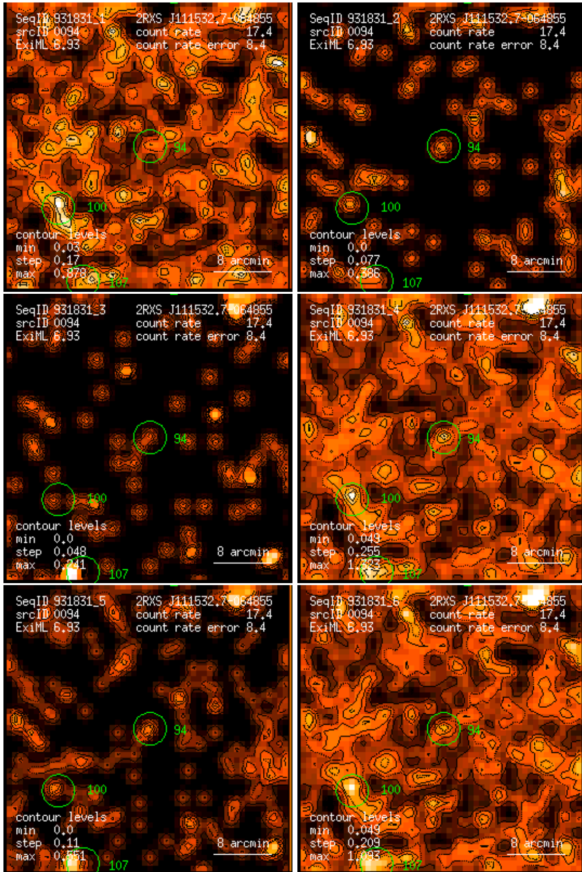
Figure 94: RASS 931831: detection 0094: band rate images, Gaussian filter: (1) PSPC channels 11 – 41, (2) 52 – 90, (3) 91 – 201, (4) 11 – 235, (5) 52 – 201, (6) 11 – 201. Broad band rates in counts/ks. Band rate contour levels in counts/ks/arcmin 2 .
