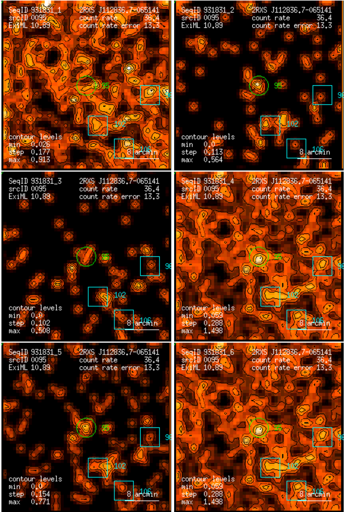
Figure 95: RASS 931831: detection 0095: band rate images, Gaussian filter: (1) PSPC channels 11 – 41, (2) 52 – 90, (3) 91 – 201, (4) 11 – 235, (5) 52 – 201, (6) 11 – 201. Broad band rates in counts/ks. Band rate contour levels in counts/ks/arcmin 2 .
