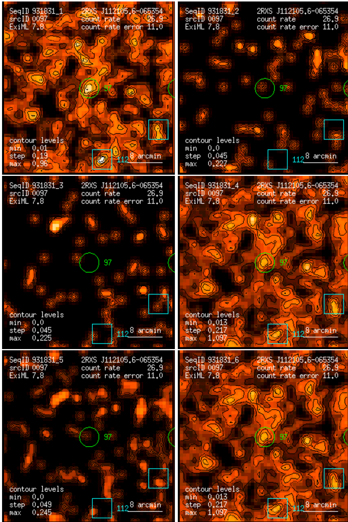
Figure 97: RASS 931831: detection 0097: band rate images, Gaussian filter: (1) PSPC channels 11 – 41, (2) 52 – 90, (3) 91 – 201, (4) 11 – 235, (5) 52 – 201, (6) 11 – 201. Broad band rates in counts/ks. Band rate contour levels in counts/ks/arcmin 2 .
